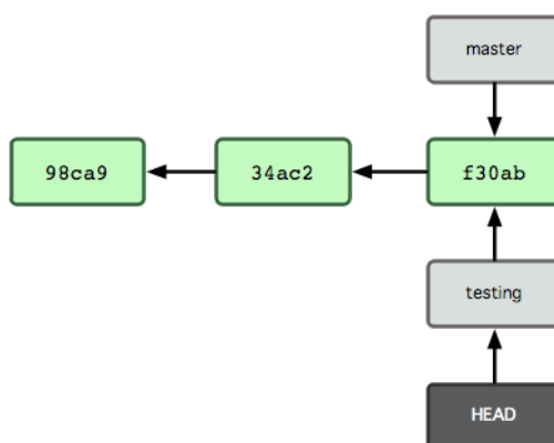
Figure 3.6: HEAD points to another branch when you switch branches.
