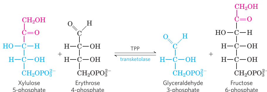
FIGURE 14-26 The second reaction catalyzed by transketolase.
