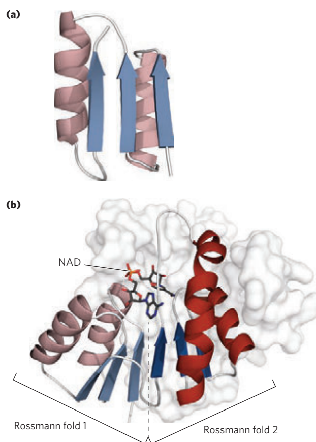
FIGURE 13–25 The Rossmann fold. This structural motif is found in the \text{NAD} -binding site of many dehydrogenases. (a) It consists of a pair of structurally similar motifs (only one of which is shown here), each having three parallel \beta sheets and two \alpha helices ( \beta - \alpha - \beta - \alpha - \beta ). (b) The nucleotide-binding domain of the enzyme lactate dehydrogenase (derived from PDB ID 3LDH) with \text{NAD} (ball-and-stick structure) bound in an extended conformation through hydrogen bonds and salt bridges to the paired \beta - \alpha - \beta - \alpha - \beta motifs of the Rossmann fold (shades of red and blue).
