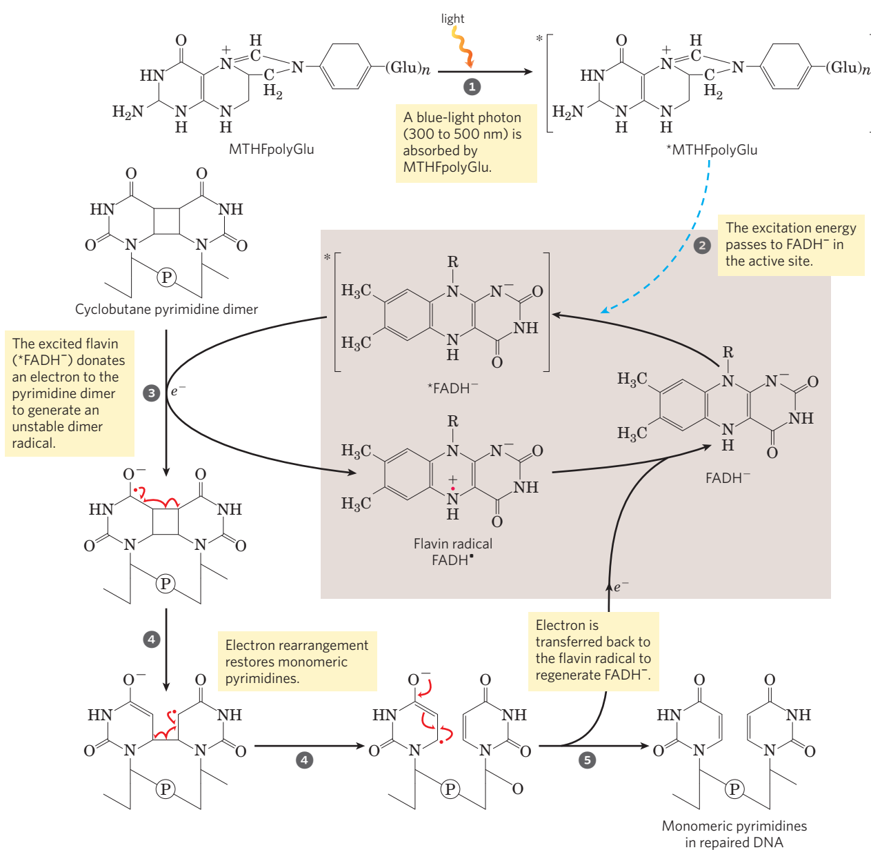
MECHANISM FIGURE 25-26 Repair of pyrimidine dimers with photolyase. Energy derived from absorbed light is used to reverse the photoreaction that caused the lesion. The two chromophores in E. coli photolyase ( M , 54,000), N 5 ,N 10 -methenyltetrahydrofolylpolyglutamate (MTHFpolyGlu) and FADH - , perform complementary functions. MTHF-
