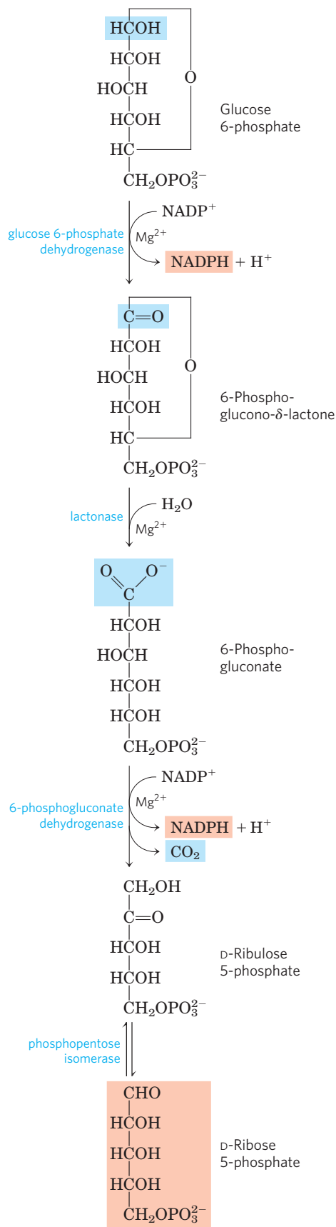
FIGURE 14-22 Oxidative reactions of the pentose phosphate pathway. The end products are ribose 5-phosphate, CO 2 , and NADPH.
