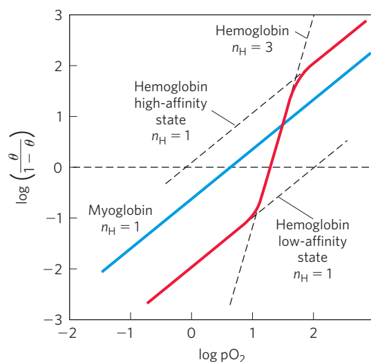
FIGURE 5-14 Hill plots for oxygen binding to myoglobin and hemoglobin. When n_H = 1 , there is no evident cooperativity. The maximum degree of cooperativity observed for hemoglobin corresponds approximately to n_H = 3 . Note that while this indicates a high level of cooperativity, n_H is less than n , the number of O_2 -binding sites in hemoglobin. This is normal for a protein that exhibits allosteric binding behavior.
