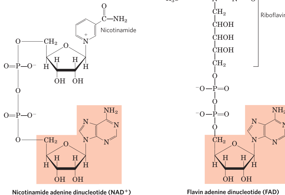
FIGURE 8-38 Some coenzymes containing adenosine. The adenosine portion is shaded in light red. Coenzyme A (CoA) functions in acyl group transfer reactions; the acyl group (such as the acetyl or acetoacetyl group) is attached to the CoA through a thioester linkage to the \beta -mercaptoethylamine moiety. NAD + functions in hydride transfers, and FAD, the active form of vitamin B 2 (riboflavin), in electron transfers. Another coenzyme incorporating adenosine is 5'-deoxyadenosylcobalamin, the active form of vitamin B 12 (see Box 17-2), which participates in intramolecular group transfers between adjacent carbons.
