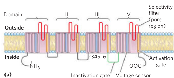
FIGURE 12-27 Voltage-gated Na + channels of neurons. Sodium channels of different tissues and organisms have a variety of subunits, but only the principal subunit ( \alpha ) is essential. (a) The \alpha subunit is a large protein with four homologous domains (I to IV, shown spread out here to illustrate the parts), each containing six transmembrane helices (1 to 6). Helix 4 in each domain (blue) is the voltage sensor; helix 6 (orange) is thought to be the activation gate. The segments between helices 5 and 6, the pore region (red), form the selectivity filter, and the segment connecting domains III and IV (green) is the inactivation gate. (b) (PDB ID 3RW0) Structure of a voltage-gated Na + channel (from the bacterium Arcobacter butzleri , but probably similar to channels of vertebrate neurons), with a funnel-shaped opening on the extracellular side, an ion selectivity filter, a central aqueous cavity, and the activation domain on the cytoplasmic side. (c) A schematic view of the Na + channel. The four domains are wrapped about a central transmembrane channel lined with polar amino acid residues. The four pore regions (red) come together near the extracellular surface to form the selectivity filter, which is conserved in all Na + channels. The filter gives the channel its ability to discriminate between Na + and other ions of similar size. The inactivation gate (green) closes (dotted lines) soon after the activation gate opens. (d) The voltage-sensing mechanism involves movement of helix 4 (blue) perpendicular to the plane of the membrane in response to a change in transmembrane potential. As shown at the top, the strong positive charge on helix 4 allows it to be pulled inward in response to the inside-negative membrane potential ( V_m ). Depolarization lessens this pull, and helix 4 relaxes by moving outward (bottom). This movement is communicated to the activation gate (orange), inducing conformational changes that open the channel.
