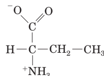
L- \alpha -Amino-n-butyric acid
