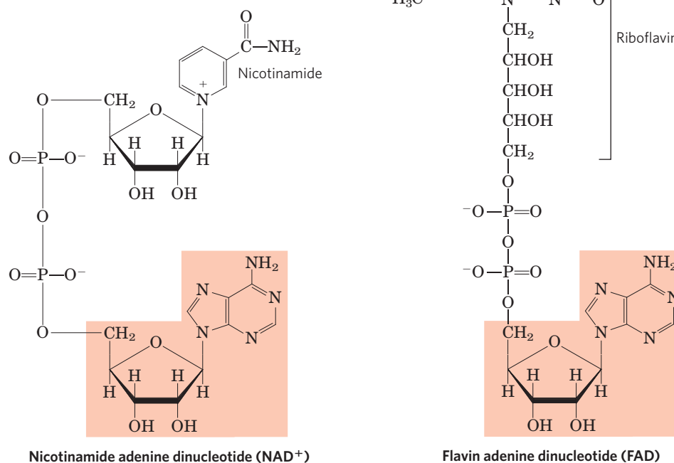
FIGURE 8-38 Some coenzymes containing adenosine. The adenosine portion is shaded in light red. Coenzyme A (CoA) functions in acyl group transfer reactions; the acyl group (such as the acetyl or acetoacetyl group) is attached to the CoA through a thioester linkage to the \beta -mercaptoethylamine moiety. NAD + functions in hydride transfers, and FAD, the active form of vitamin B 2 (riboflavin), in electron transfers. Another coenzyme incorporating adenosine is 5'-deoxyadenosylcobalamin, the active form of vitamin B 12 (see Box 17-2), which participates in intramolecular group transfers between adjacent carbons.
