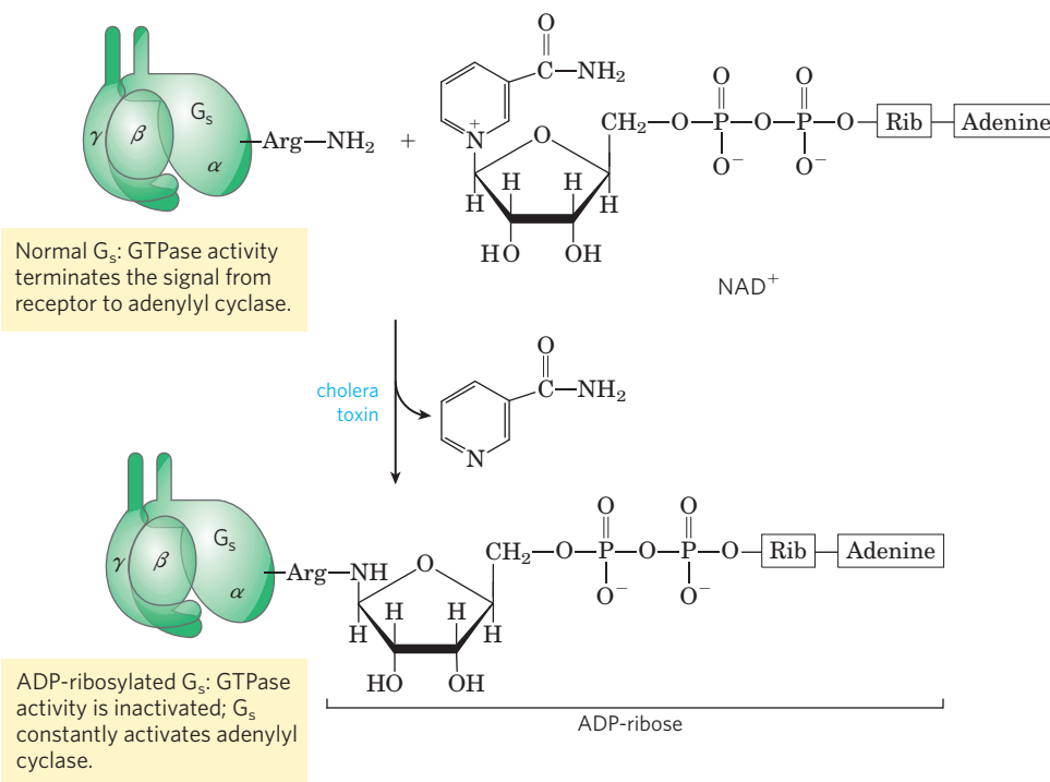
FIGURE 5 The bacterial toxins that cause cholera and whooping cough (pertussis) are enzymes that catalyze transfer of the ADP-ribose moiety of \text{NAD}^+ to an Arg residue of G_s (in the case of cholera toxin, as shown here) or a Cys residue of G_i (pertussis toxin). The G proteins thus modi-
