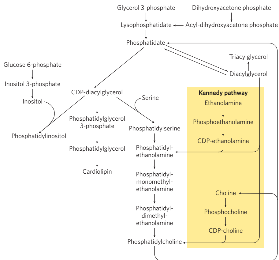
FIGURE 21-28 Summary of the pathways for synthesis of major phospholipids and triacylglycerides in a eukaryote (yeast). Phosphatidic acid is formed by transacylation of L-glycerol 3-phosphate with two fatty acyl groups donated from fatty acyl-CoA. The enzyme phosphatidic acid phosphatase (lipin) converts phosphatidic acid to diacylglycerol, which in the Kennedy pathway condenses with a CDP-activated head group (ethanolamine or choline) to form phosphatidylethanolamine or phosphatidylcholine. Alternatively, phosphatidic acid can be activated with a CDP moiety, which is displaced by condensation with a head group alcohol—inositol, glycerol 3-phosphate, or serine, forming phosphatidylinositol, phosphatidylglycerol, or phosphatidylserine. Decarboxylation of phosphatidylserine yields phosphatidylethanolamine, and methylation of phosphatidylethanolamine produces phosphatidylcholine. Not shown here are the head-group exchange reactions (see Fig. 21-29a) that interconvert phosphatidylethanolamine, phosphatidylserine, and phosphatidylcholine in mammals. Lysophosphatidic acid is phosphatidic acid missing one of the two fatty acyl groups.
