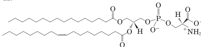
Phosphatidylserine
