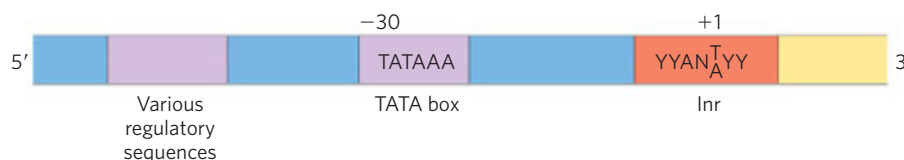
FIGURE 26-8 Some common sequences in promoters recognized by eukaryotic RNA polymerase II. The TATA box is the major assembly point for the proteins of the preinitiation complexes of Pol II. The DNA is unwound at the initiator sequence (Inr), and the transcription start site is usually within or very near this sequence. In the Inr consensus sequence shown here, N represents any nucleotide; Y, a pyrimidine nucleotide. Many additional sequences serve as binding sites for a wide variety of proteins that affect the activity of Pol II. These sequences are important in regulating Pol II promoters and differ greatly in type and number, and
