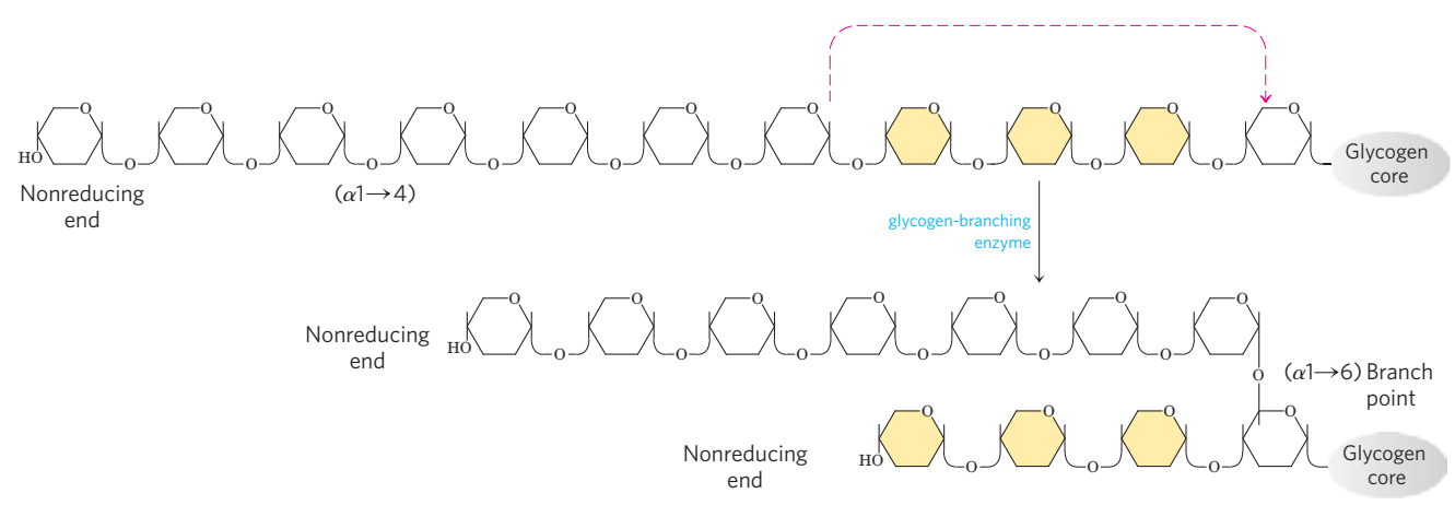
FIGURE 15-33 Branch synthesis in glycogen. The glycogen-branching enzyme (also called amylo (1→4) to (1→6) transglycosylase, or
