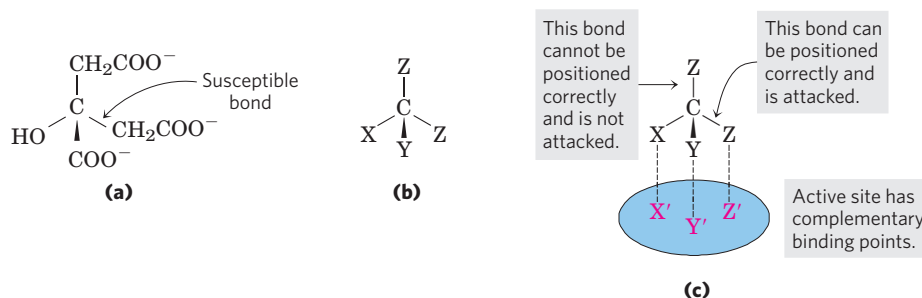
FIGURE 2 The prochiral nature of citrate. (a) Structure of citrate; (b) schematic representation of citrate: X = -OH; Y = \text{COO}^- ; Z = \text{-CH}_2\text{COO}^- . (c) Correct complementary fit of citrate to the binding
