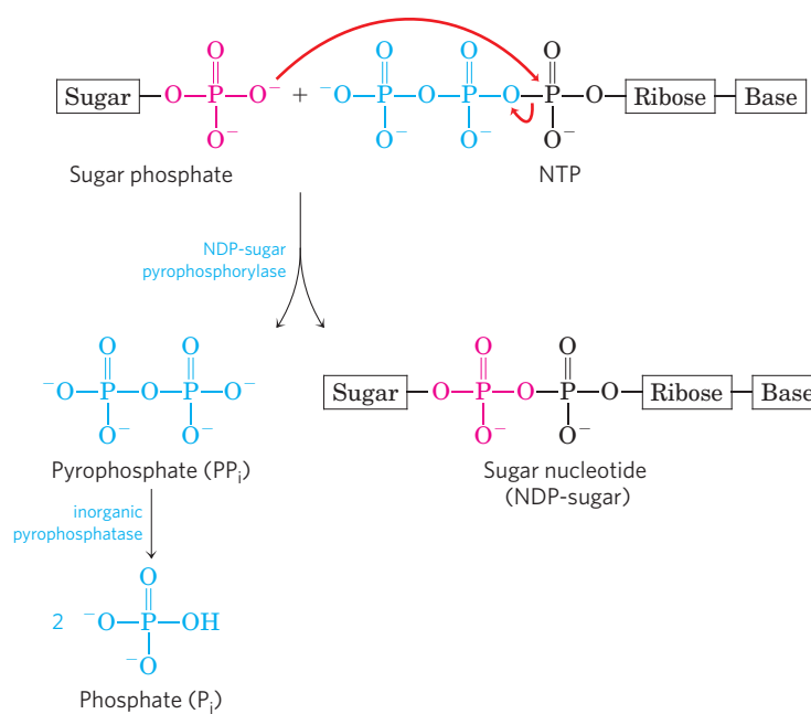
FIGURE 15-31 Formation of a sugar nucleotide. A condensation reaction occurs between a nucleoside triphosphate (NTP) and a sugar phosphate. The negatively charged oxygen on the sugar phosphate serves as a nucleophile, attacking the \alpha phosphate of the nucleoside triphosphate and displacing pyrophosphate. The reaction is pulled in the forward direction by the hydrolysis of PP_i by inorganic pyrophosphatase.
