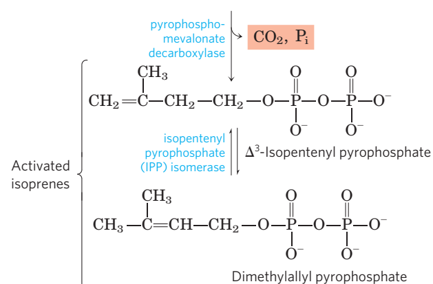
FIGURE 21-35 Conversion of mevalonate to activated isoprene units. Six of these activated units combine to form squalene (see Fig. 21-36). The leaving groups of 3-phospho-5-pyrophosphomevalonate are shaded light red. The bracketed intermediate is hypothetical.
