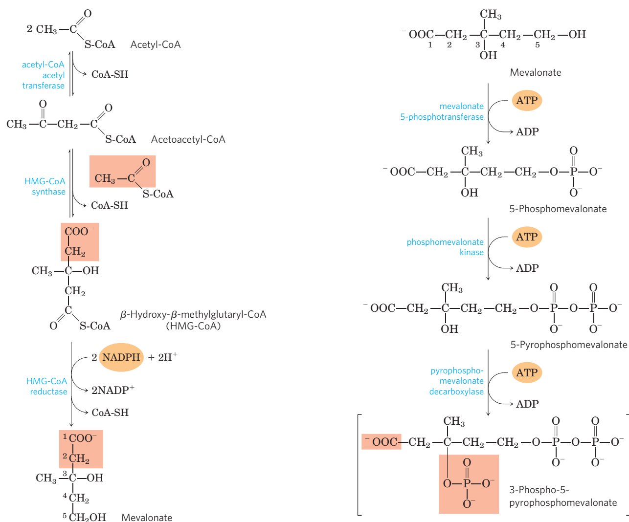
FIGURE 21-34 Formation of mevalonate from acetyl-CoA. The origin of C-1 and C-2 of mevalonate from acetyl-CoA is shaded light red.
