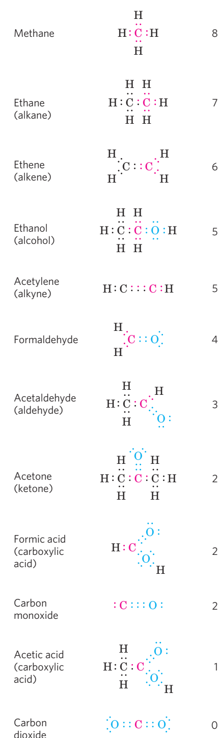
FIGURE 13–22 Different levels of oxidation of carbon compounds in the biosphere. To approximate the level of oxidation of these compounds, focus on the red carbon atom and its bonding electrons. When this carbon is bonded to the less electronegative H atom, both bonding electrons (red) are assigned to the carbon. When carbon is bonded to another carbon, bonding electrons are shared equally, so one of the two electrons is assigned to the red carbon. When the red carbon is bonded to the more electronegative O atom, the bonding electrons are assigned to the oxygen. The number to the right of each compound is the number of electrons “owned” by the red carbon, a rough expression of the degree of oxidation of that compound. As the red carbon undergoes oxidation (loses electrons), the number gets smaller.
