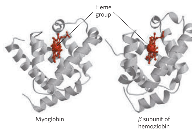
FIGURE 5-6 Comparison of the structures of myoglobin (PDB ID 1MBO) and the β subunit of hemoglobin (derived from PDB ID 1HGA).
