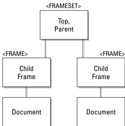
Figure 11-2: Two-frame window and document hierarchy
