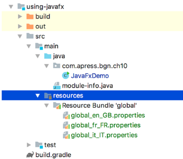
Figure 10-10. Resource Bundle with three resource files
