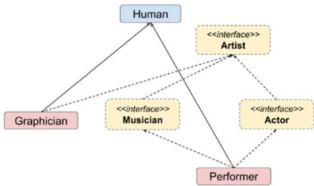
Figure 6-1. The Performer hierarchy
