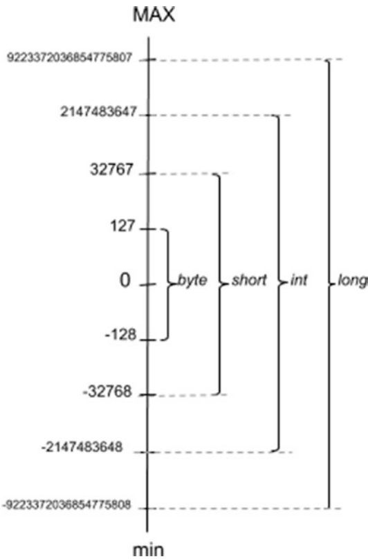
Figure 5-8. Java numeric types to represent integer values
