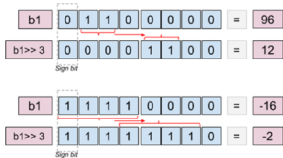
Figure 6-7. The effect of the >>> operator
