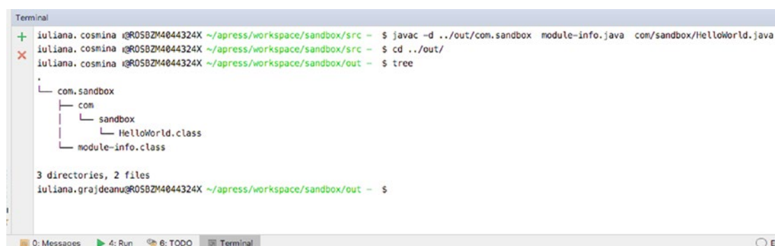
Figure 3-22. Java module com.sandbox compiled manually
