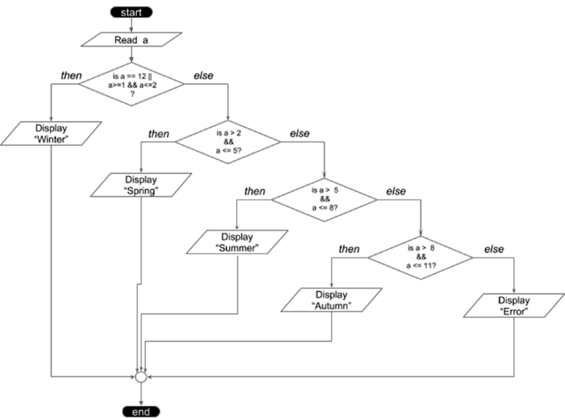
Figure 7-4. Complex if-else flowchart sample
