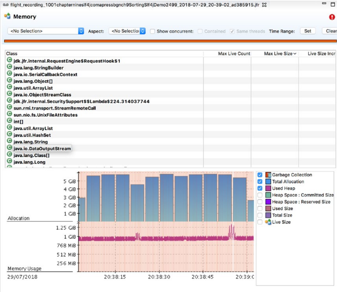
Figure 9-11. JMX console ➤ the Memory tab
