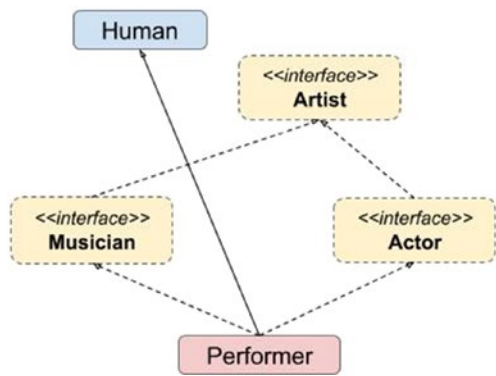
Figure 4-9. Java hierarchy with more interfaces for Performer class
