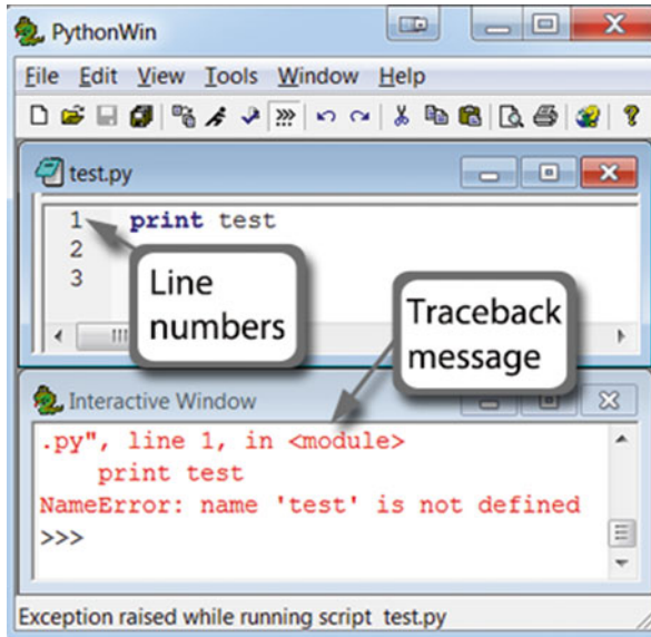
Figure 4.2 Exception raised.
