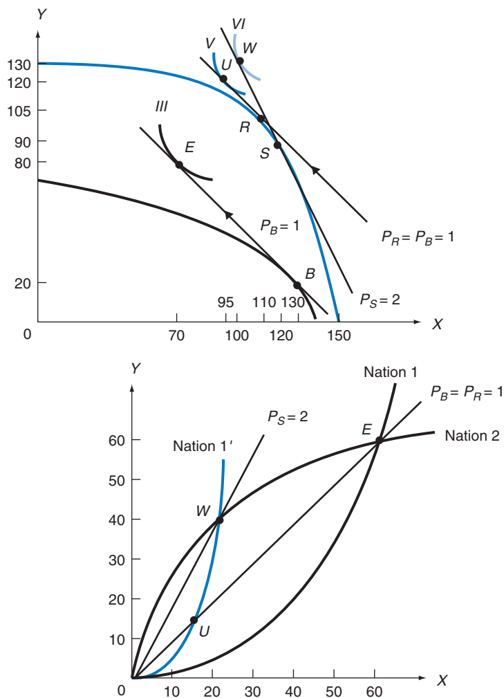
FIGURE 7.7. Growth That Improves Nation 1's Terms of Trade and Welfare. If K (Nation 1's scarce factor) doubled in Nation 1, production would take place at point R at the unchanged terms of trade of P_R = P_B = 1 (see the top panel). Nation 1 would exchange 15 X for 15 Y with Nation 2 and consume at point U on indifference curve V . However, if Nation 1 is large, its terms of trade will improve because it is willing to export less of X at P_R = P_B = 1 . At P_S = 2 , Nation 1 produces at point S , exchanges 20 X for 40 Y with Nation 2, and consumes at point W on indifference curve VI . Nation 1's welfare increases because of both favorable wealth and terms-of-trade effects. The bottom panel shows with offer curves the effect of this type of growth on the volume and the terms of trade when Nation 1 does not and when it does affect its terms of trade. Compare this to Figure 7.5.
