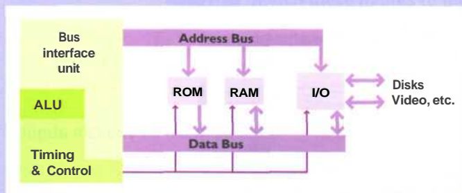
Fig 3 Computer buses
