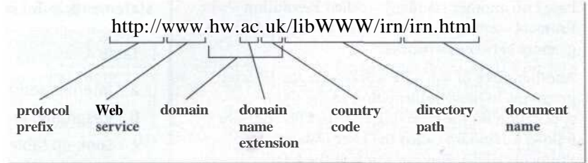
Fig 1 Uniform Resource Locator
