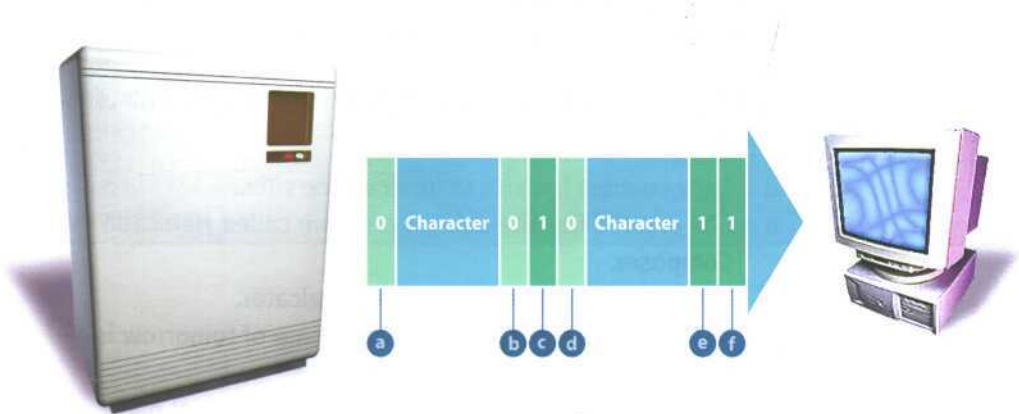
Fig3 Asynchronous transmission
