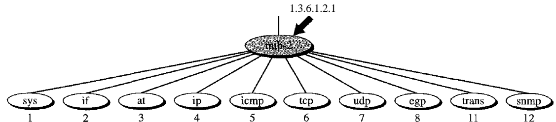
Figure 28.15 mib-2
