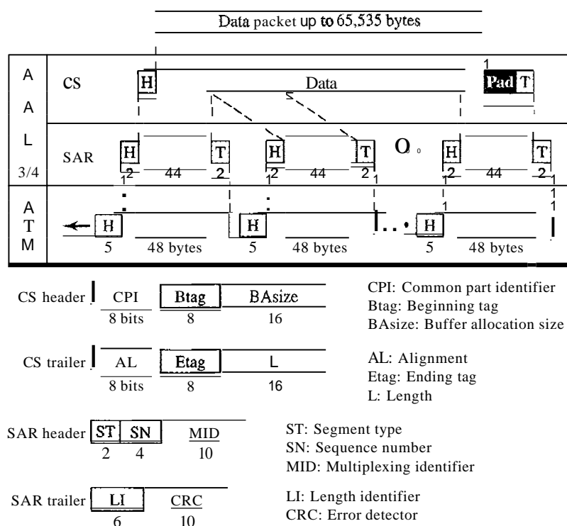
Figure 18.22 AAL3/4
