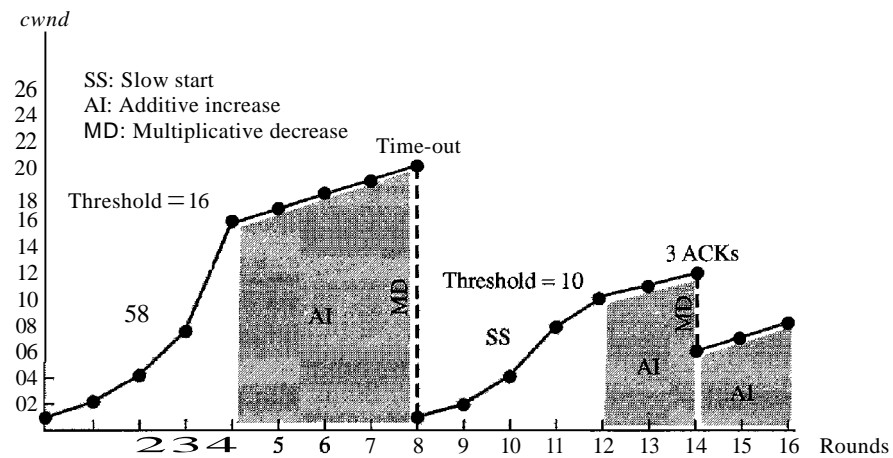
Figure 24.11 Congestion example
