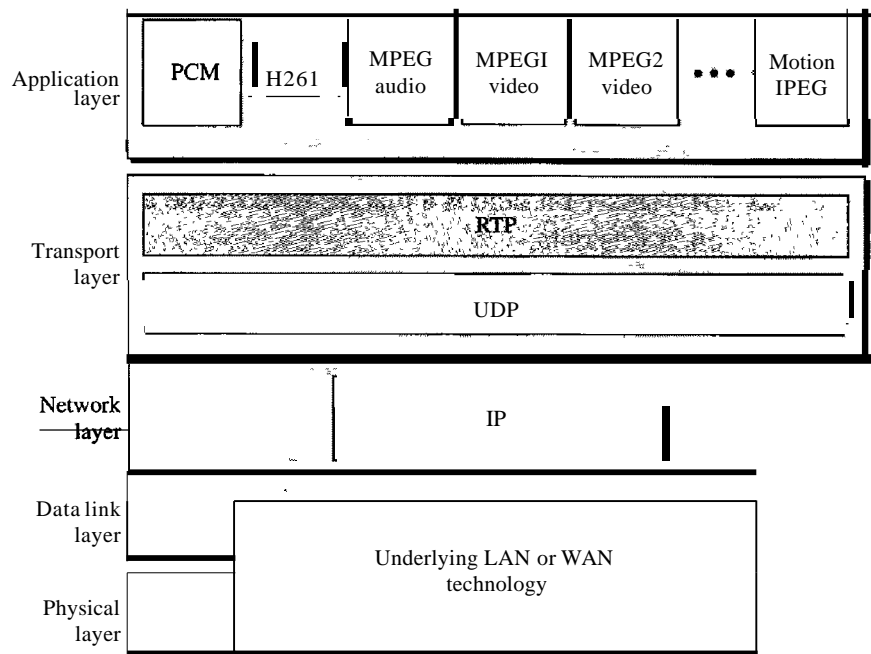
Figure 29.18 RTP
