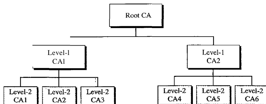
Figure 31.27 PKI hierarchy
