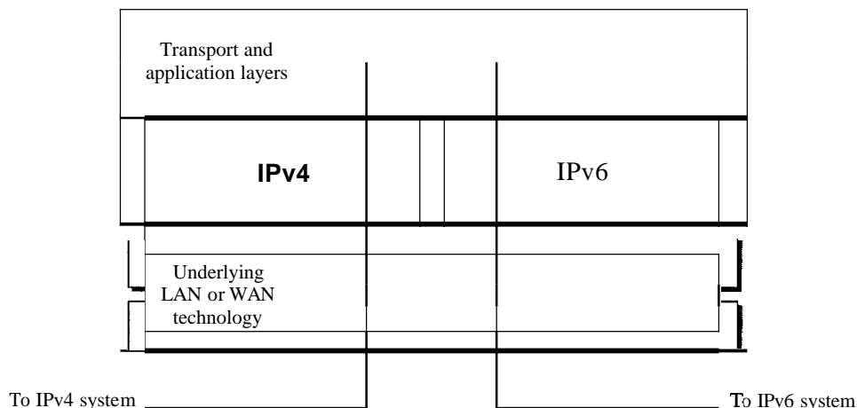
Figure 20.19 Dual stack
