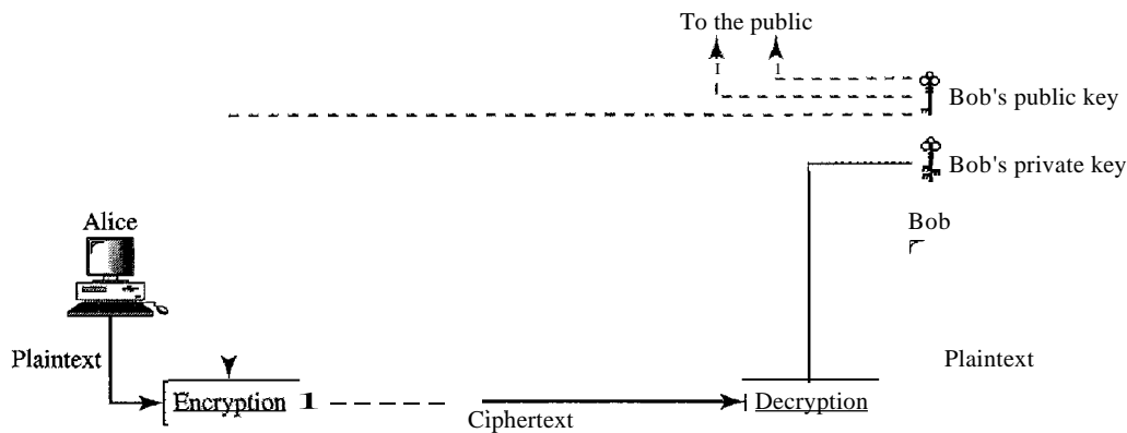
Figure 30.4 Asymmetric-key cryptography
