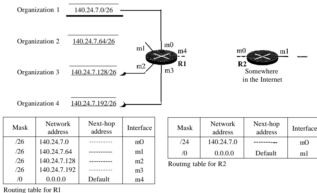
Figure 22.7 Address aggregation
