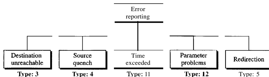
Figure 21.9 Error-reporting messages
