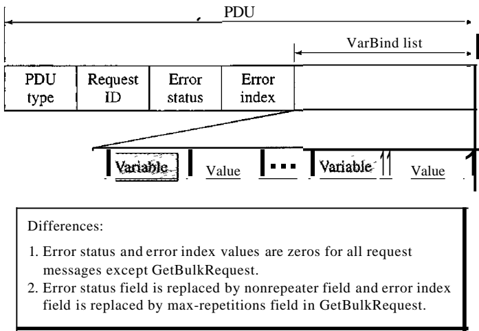
Figure 28.21 SNMP PDUformat
