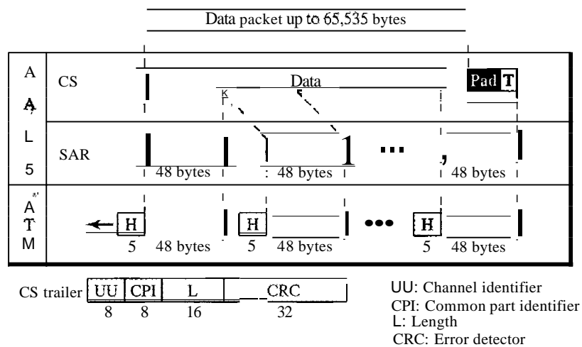
Figure 18.23 AAL5
