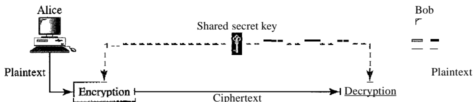
Figure 30.3 Symmetric-key cryptography
