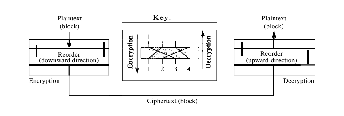
Figure 30.8 Transposition cipher
