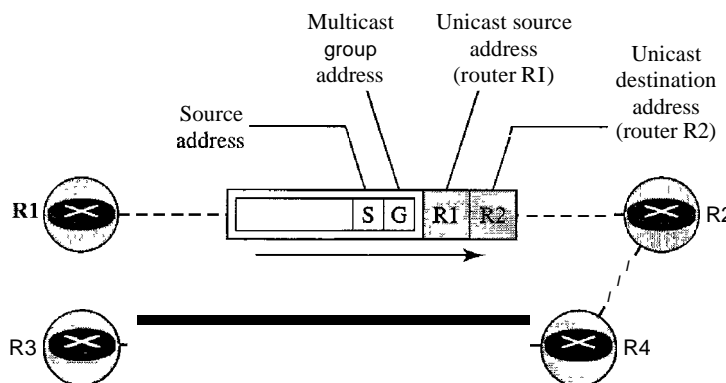
Figure 22.47 MBONE
