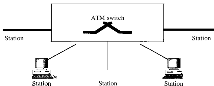
Figure 18.25 Pure ATMLAN
