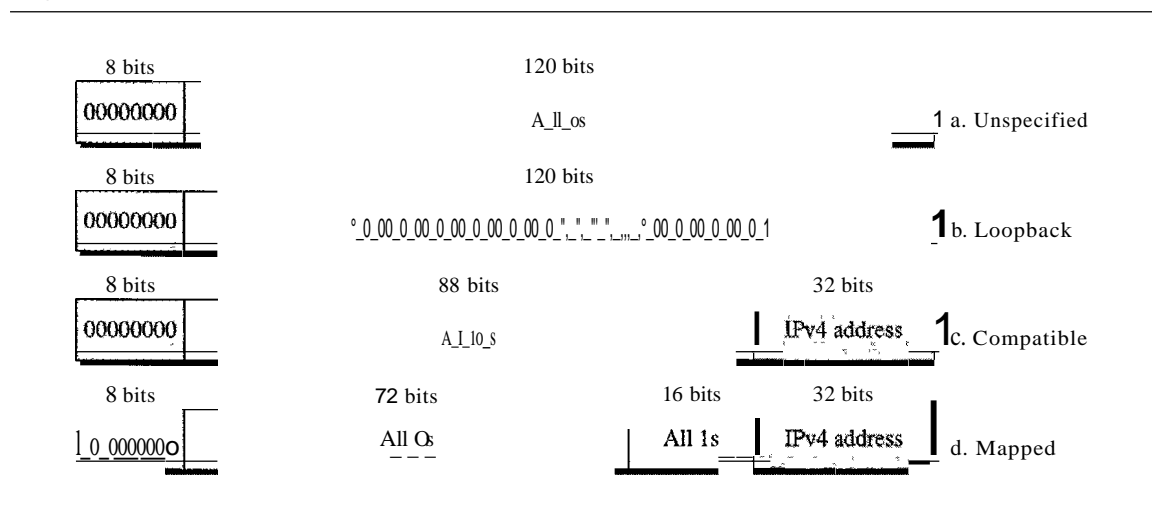
Figure 19.18 Reserved addresses in IPv6
