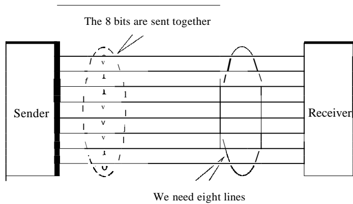
Figure 4.32 Parallel transmission
