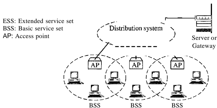
Figure 14.2 Extended service sets (ESSs)
