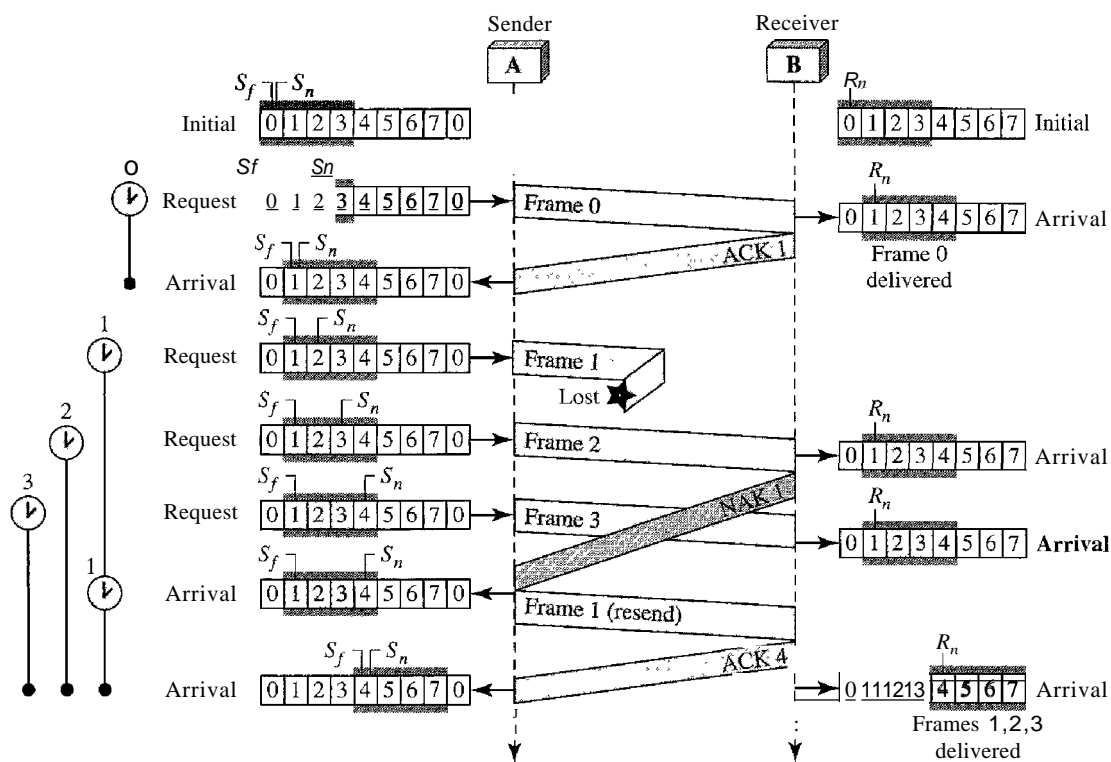
Figure 11.23 Flow diagram for Example 11.8
