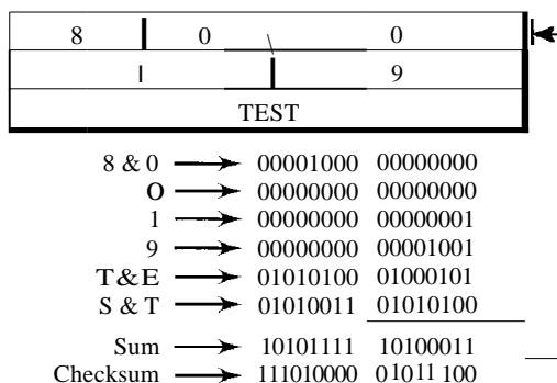
Figure 21.14 Example of checksum calculation
