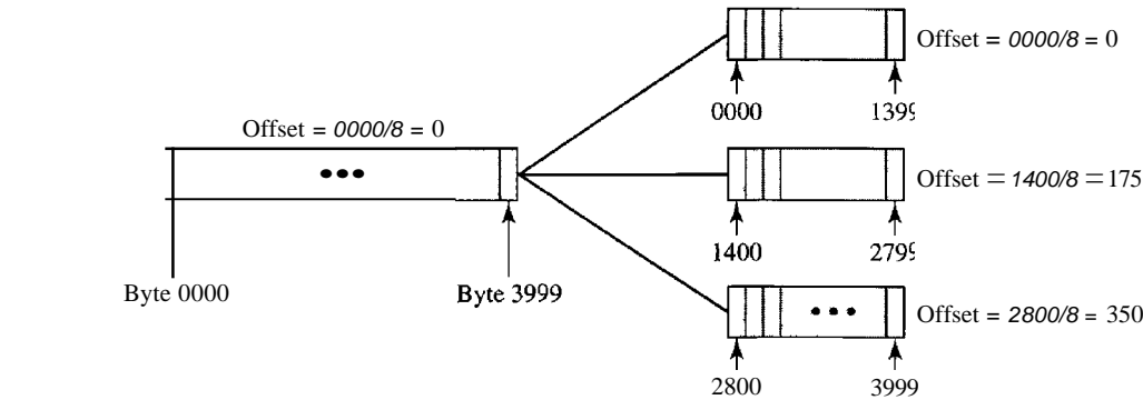
Figure 20.11 Fragmentation example
