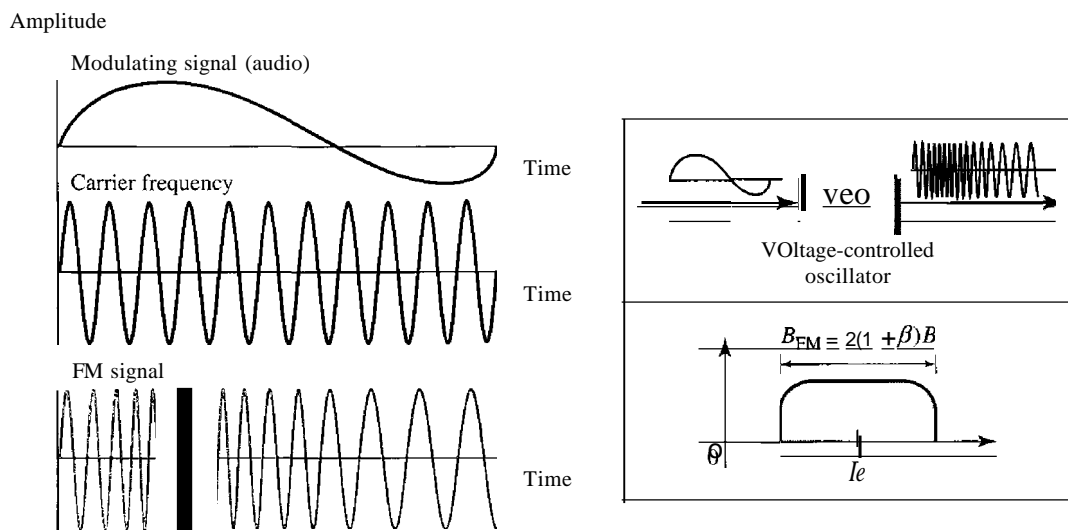
Figure 5.18 Frequency modulation
