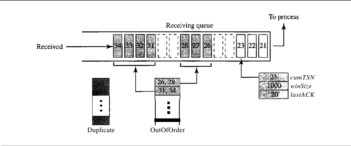
Figure 23.39 Error control, receiver site
