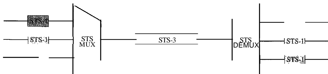
Figure 17.12 STS multiplexing/demultiplexing
