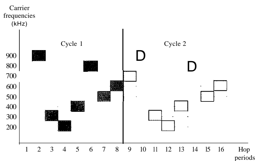
Figure 6.30 FHSS cycles
