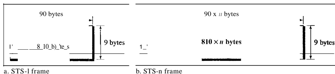
Figure 17.4 An STS-1 and an STS-n frame
