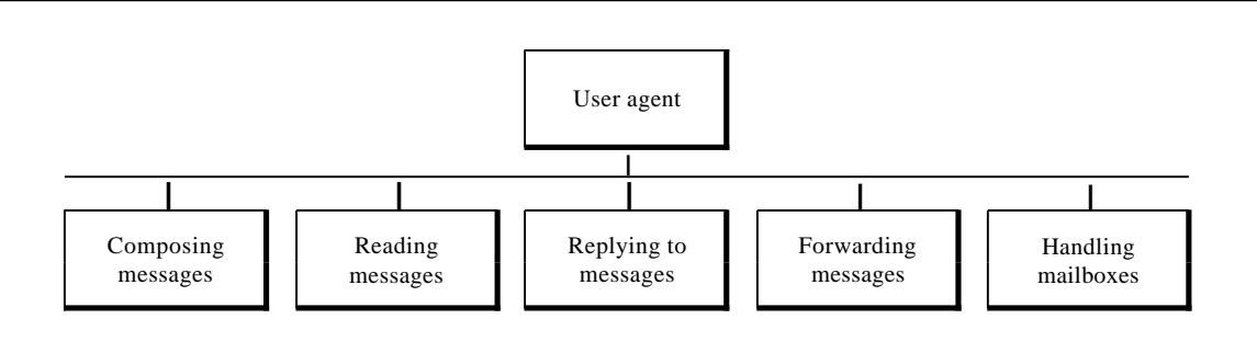
Figure 26.11 Services of user agent
