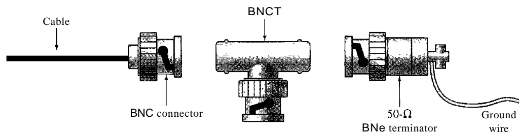
Figure 7.8 BNC connectors
