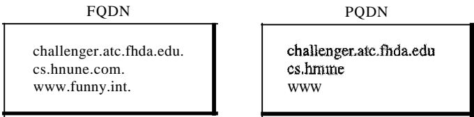
Figure 25.4 FQDN and PQDN
