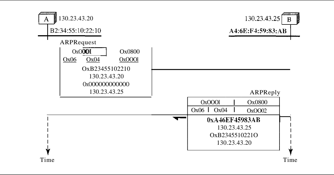
Figure 21.5 Example 21.1, an ARP request and reply
