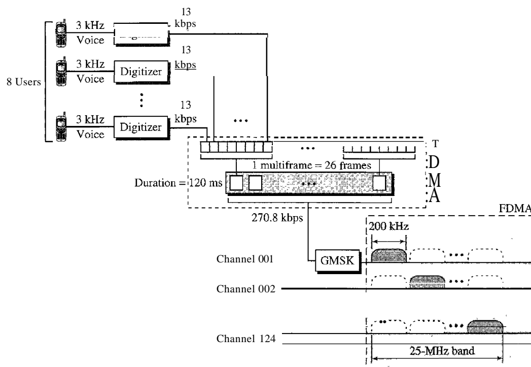
Figure 16.8 GSM
