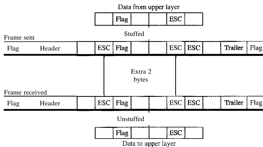
Figure 11.2 Byte stuffing and unstuffing
