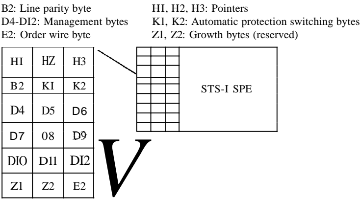
Figure 17.8 STS-1 frame: line overhead
