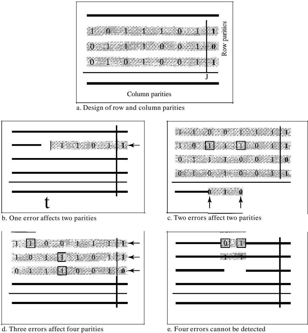
Figure 10.11 Two-dimensional parity-check code
