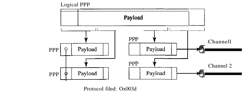
Figure 11.40 Multilink PPP
