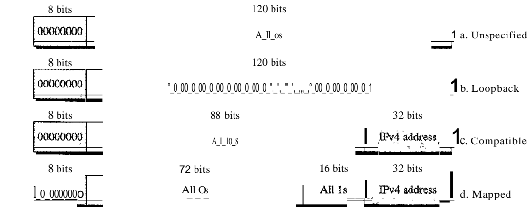
Figure 19.18 Reserved addresses in IPv6
