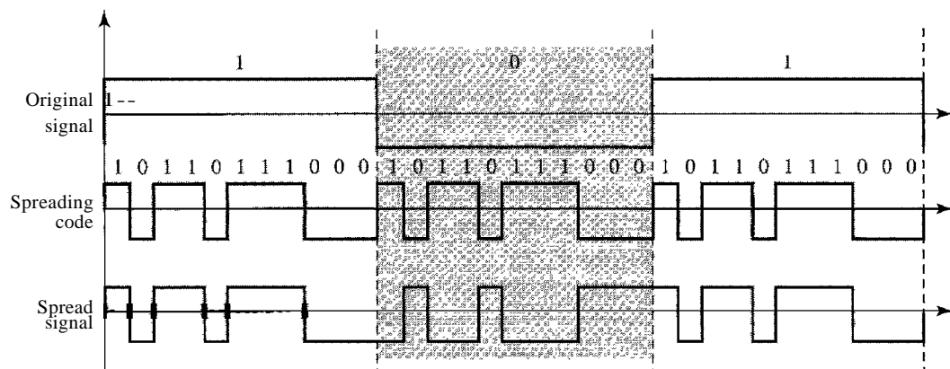
Figure 6.33 DSSS example
