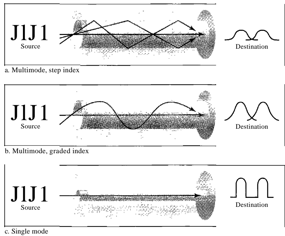
Figure 7.13 Modes
