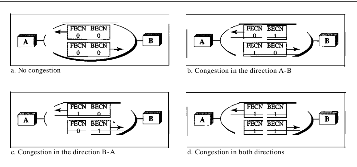
Figure 24.14 Four cases of congestion
