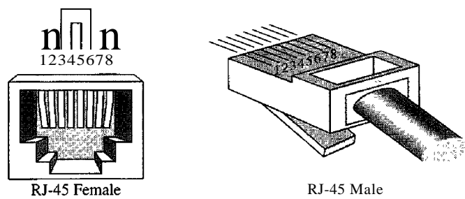
Figure 7.5 UTP connector
