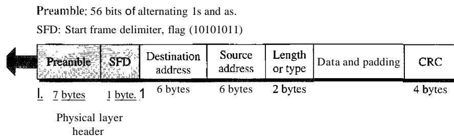
Figure 13.4 802.3 MAC frame
