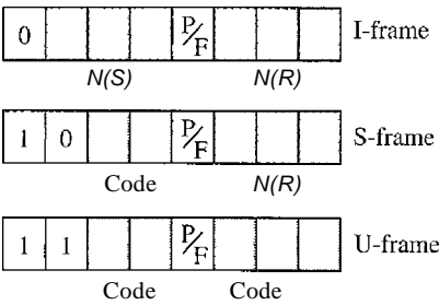
Figure 11.28 Control field format for the different frame types
