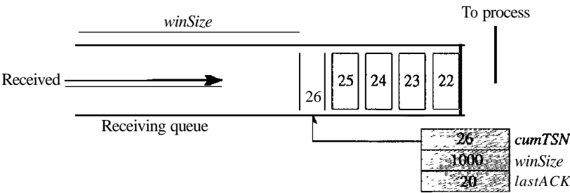
Figure 23.36 Flow control, receiver site
