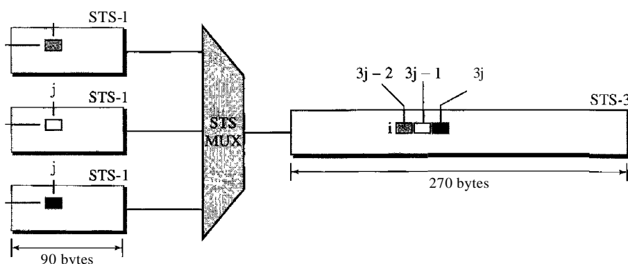
Figure 17.13 Byte interleaving
