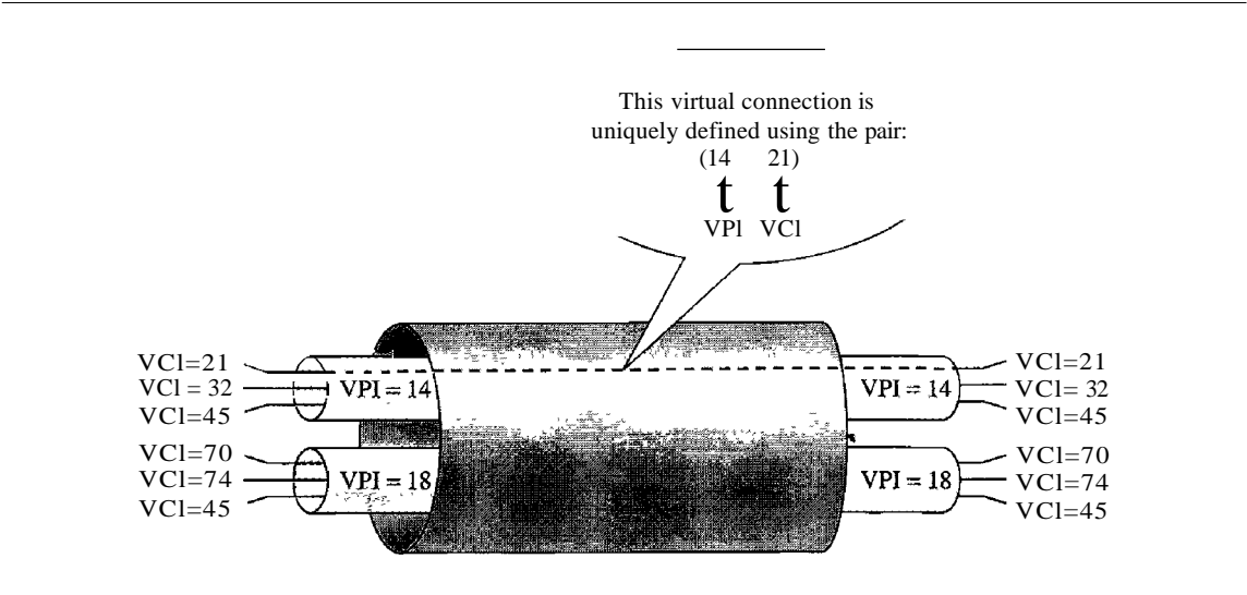
Figure 18.12 Connection identifiers
