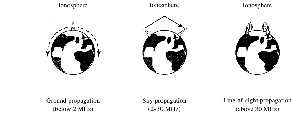
Figure 7.18 Propagation methods
