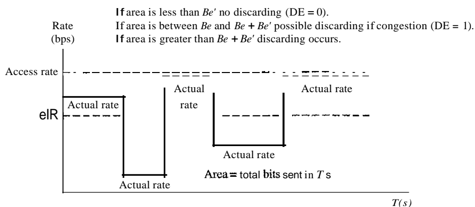
Figure 24.29 User rate in relation to Be and Be + Be'
