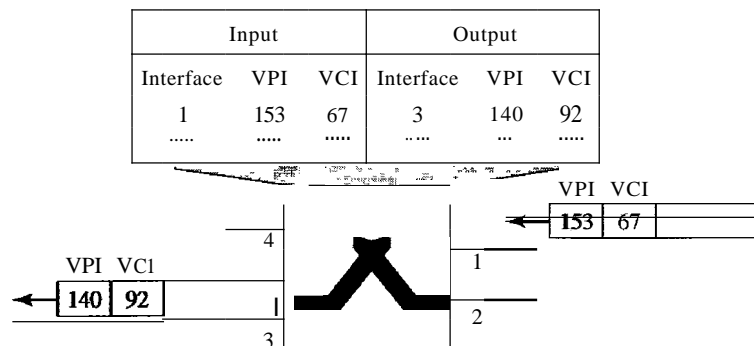
Figure 18.15 Routing with a switch
