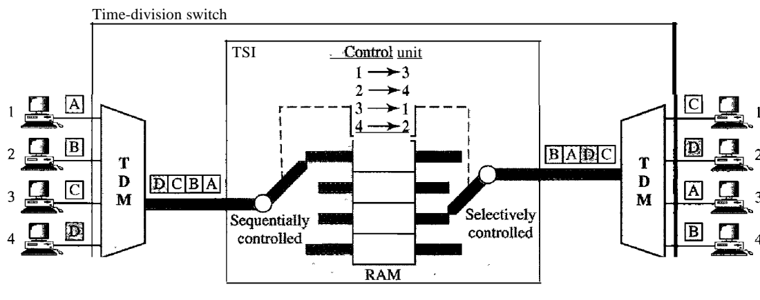
Figure 8.19 Time-slot interchange
