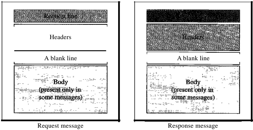
Figure 27.13 Request and response messages
