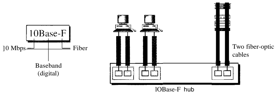
Figure 13.13 IOBase-F implementation
