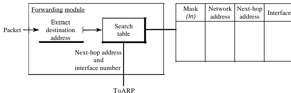
Figure 22.5 Simplified forwarding module in classless address
