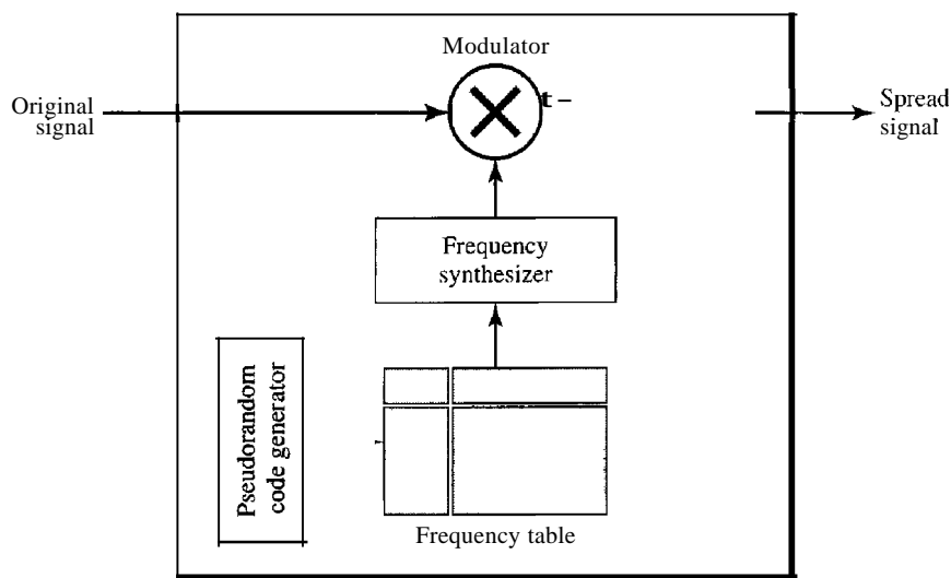
Figure 6.28 Frequency hopping spread spectrum (FHSS)
