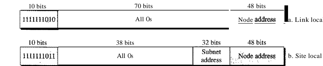
Figure 19.19 Local addresses in IPv6
