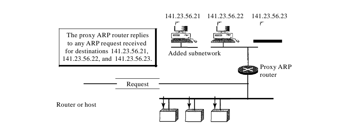
Figure 21.6 Proxy ARP
