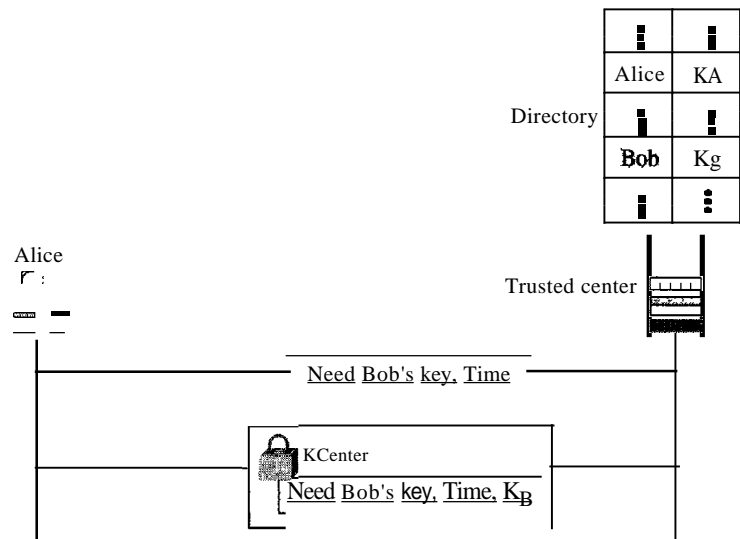
Figure 31.25 Controlled trusted center
