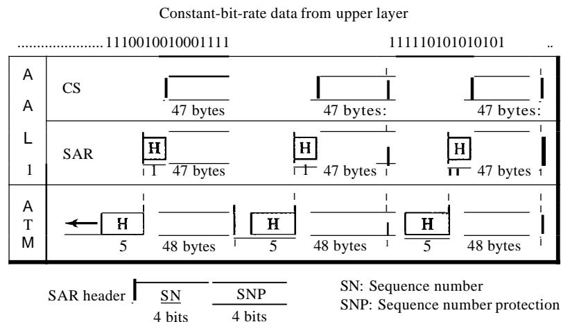
Figure 18.20 AAL1
