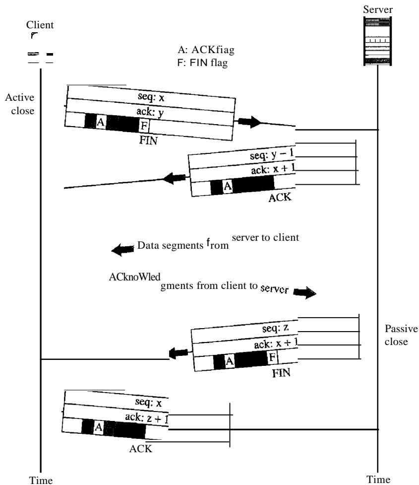
Figure 23.21 Half-close
