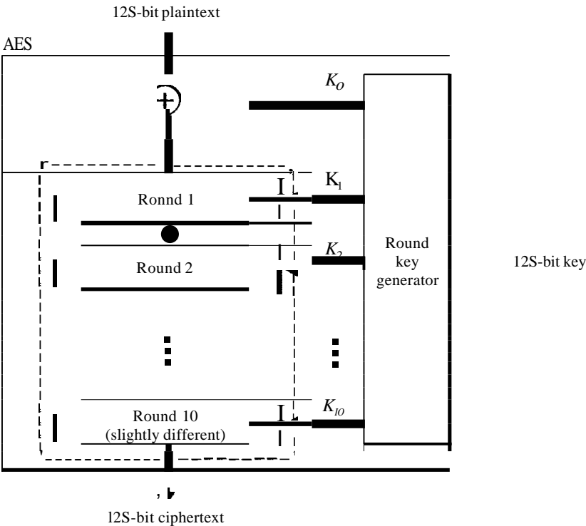
Figure 30.17 AES
