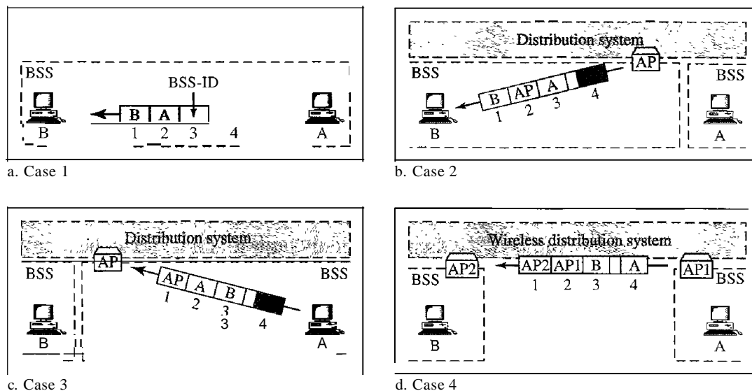
Figure 14.9 Addressing mechanisms
