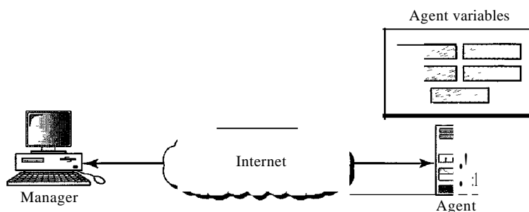
Figure 28.2 SNMP concept
