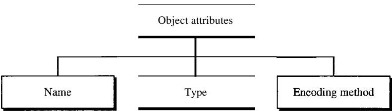
Figure 28.5 Object attributes
