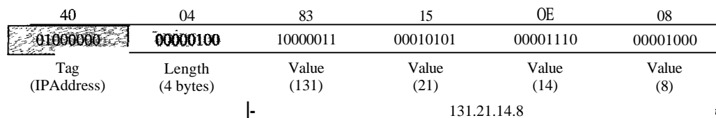
Figure 28.14 Example 28.4, IPAddress 131.21.14.8
