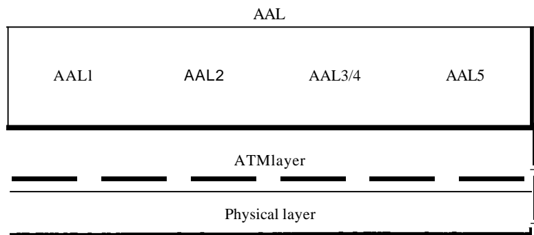
Figure 18.16 ATM layers
