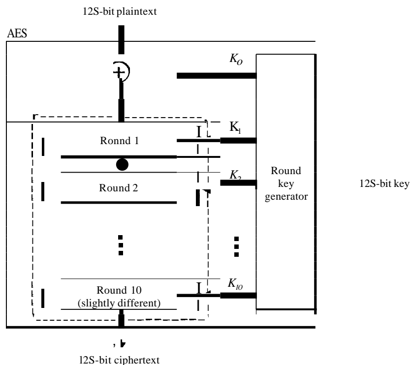
Figure 30.17 AES
