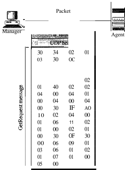
Figure 28.24 GetRequest message
