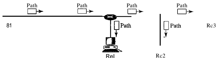
Figure 24.22 Path messages
