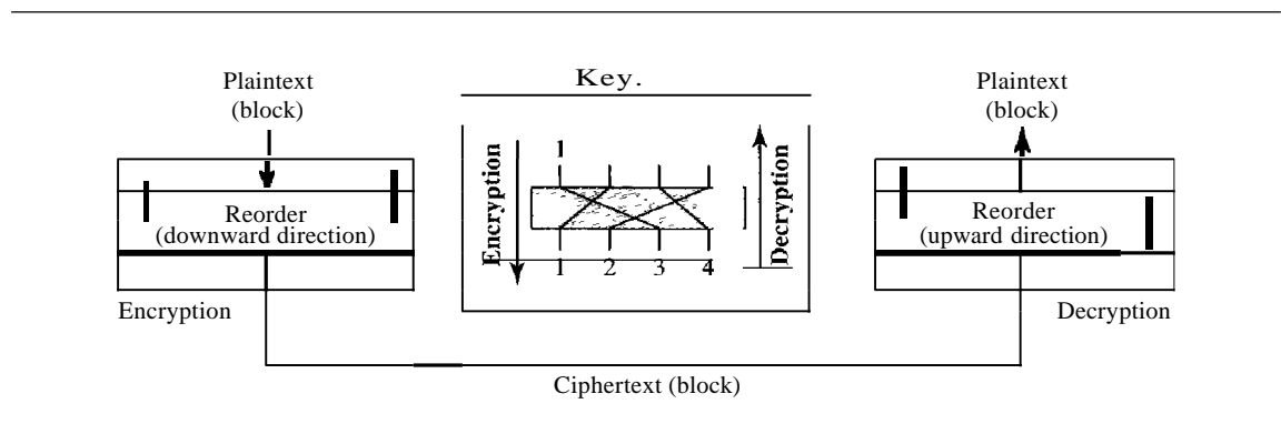
Figure 30.8 Transposition cipher
