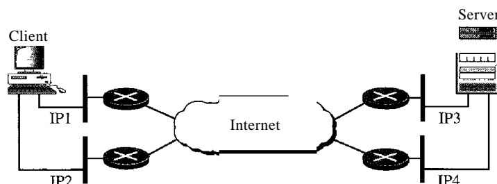
Figure 23.28 Multihoming concept
