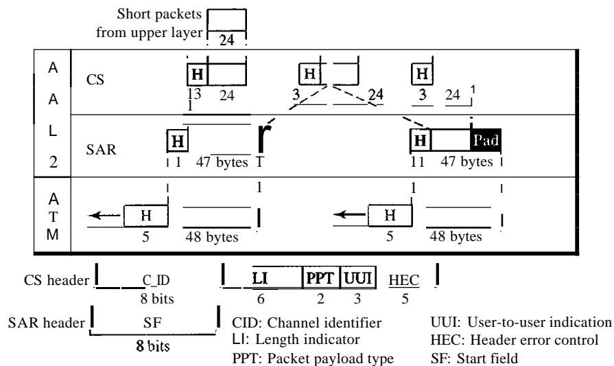
Figure 18.21 AAL2
