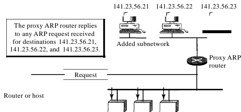
Figure 21.6 Proxy ARP
