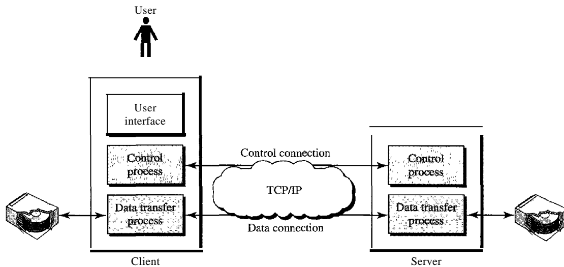
Figure 26.21 FTP
