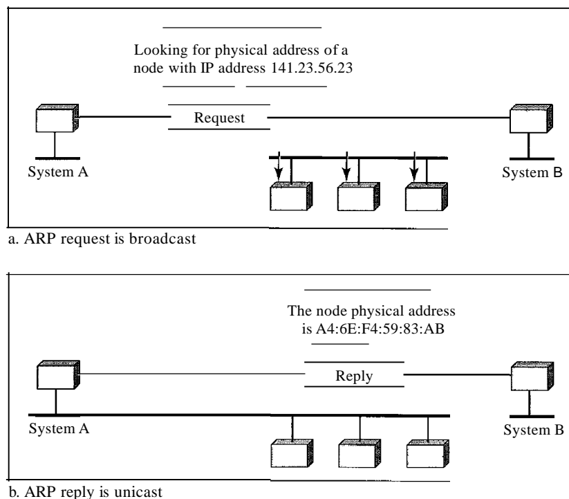
Figure 21.1 ARP operation
