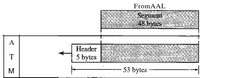
Figure 18.18 ATM layer
