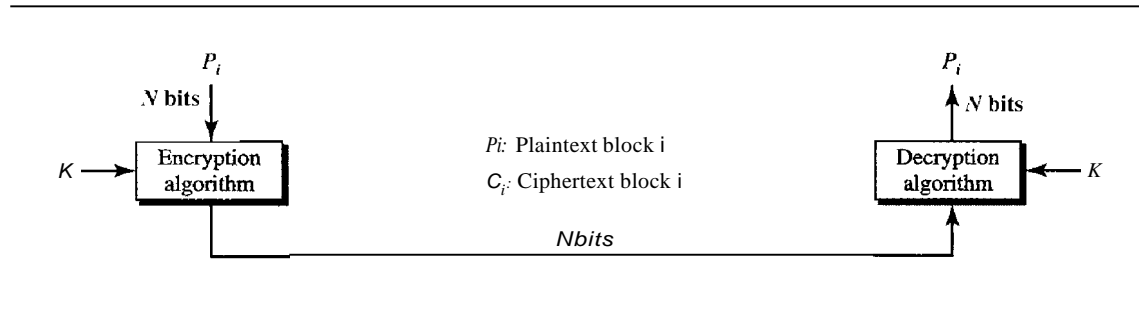
Figure 30.20 ECB mode
