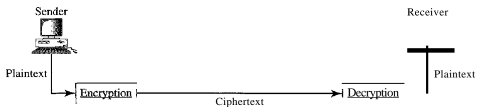
Figure 30.1 Cryptography components
