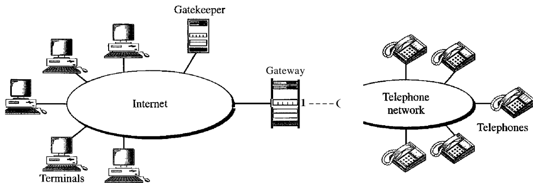
Figure 29.25 H.323 architecture
