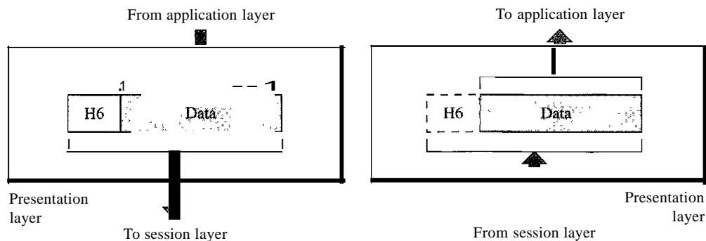
Figure 2.13 Presentation layer
