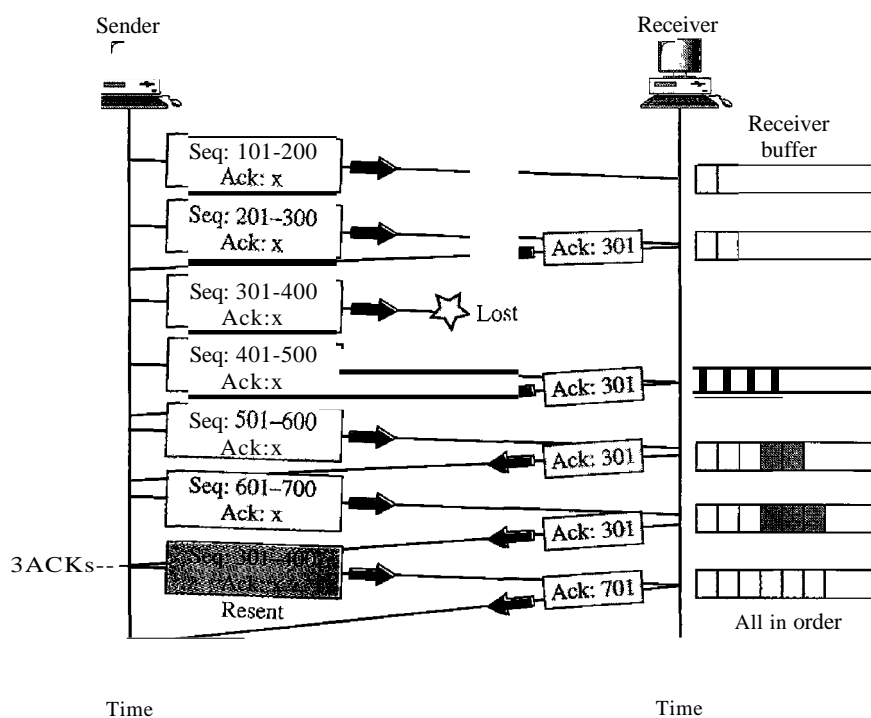
Figure 23.26 Fast retransmission
