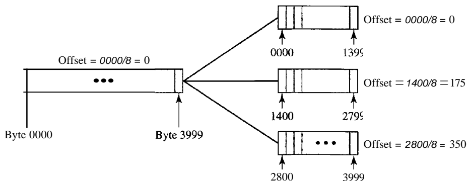
Figure 20.11 Fragmentation example
