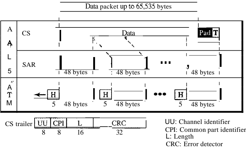
Figure 18.23 AAL5
