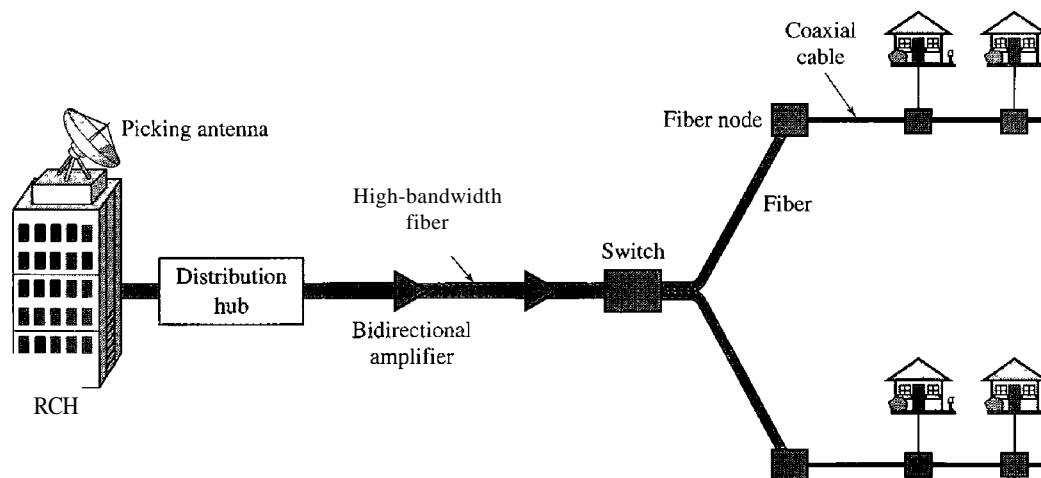
Figure 9.15 Hybridfiber-coaxial (HFC) network
