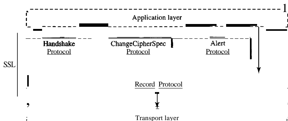
Figure 32.16 Four SSL protocols
