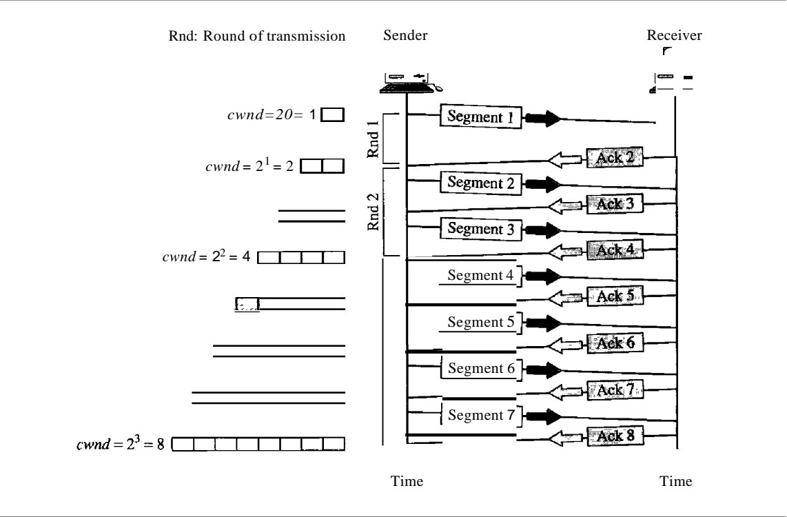
Figure 24.8 Slow start, exponential increase
