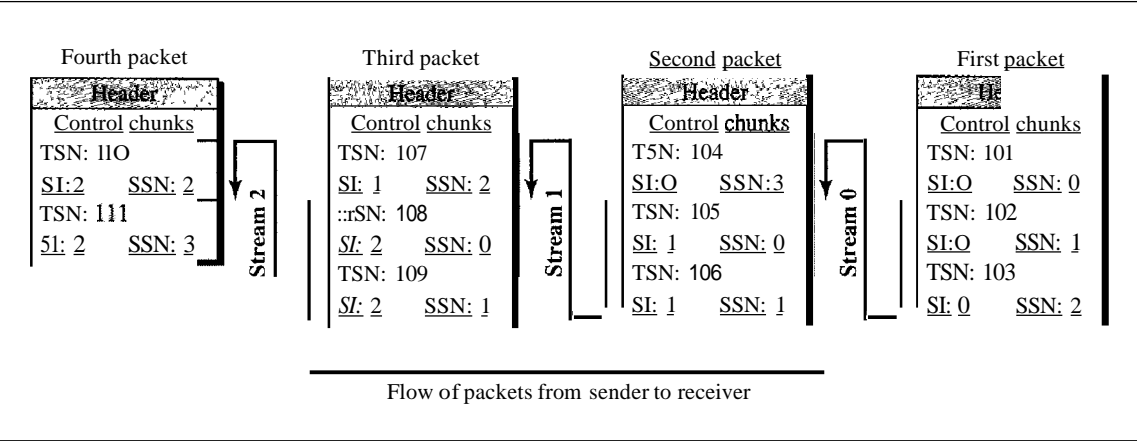
Figure 23.30 Packet, data chunks, and streams
