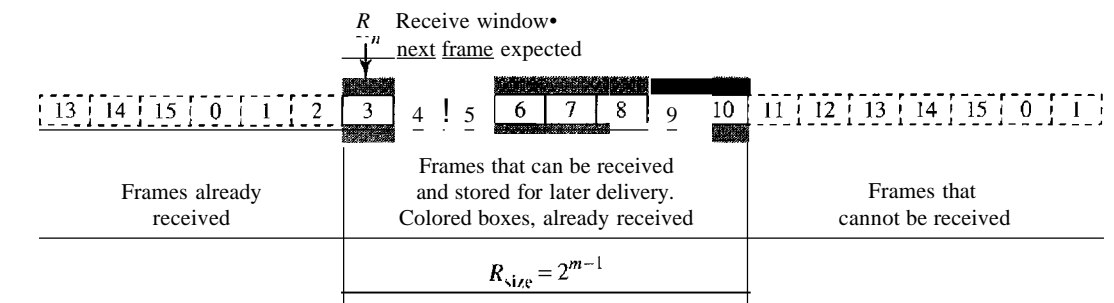
Figure 11.19 Receive window for Selective Repeat ARQ
