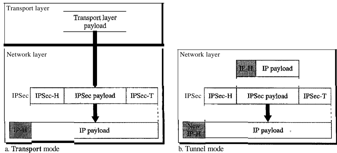
Figure 32.3 Transport mode and tunnel modes ofIPSec protocol
