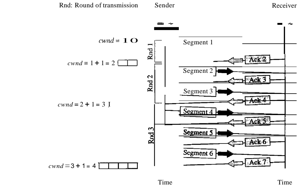
Figure 24.9 Congestion avoidance, additive increase
