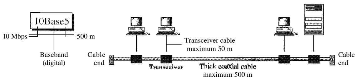
Figure 13.10 10Base5 implementation
