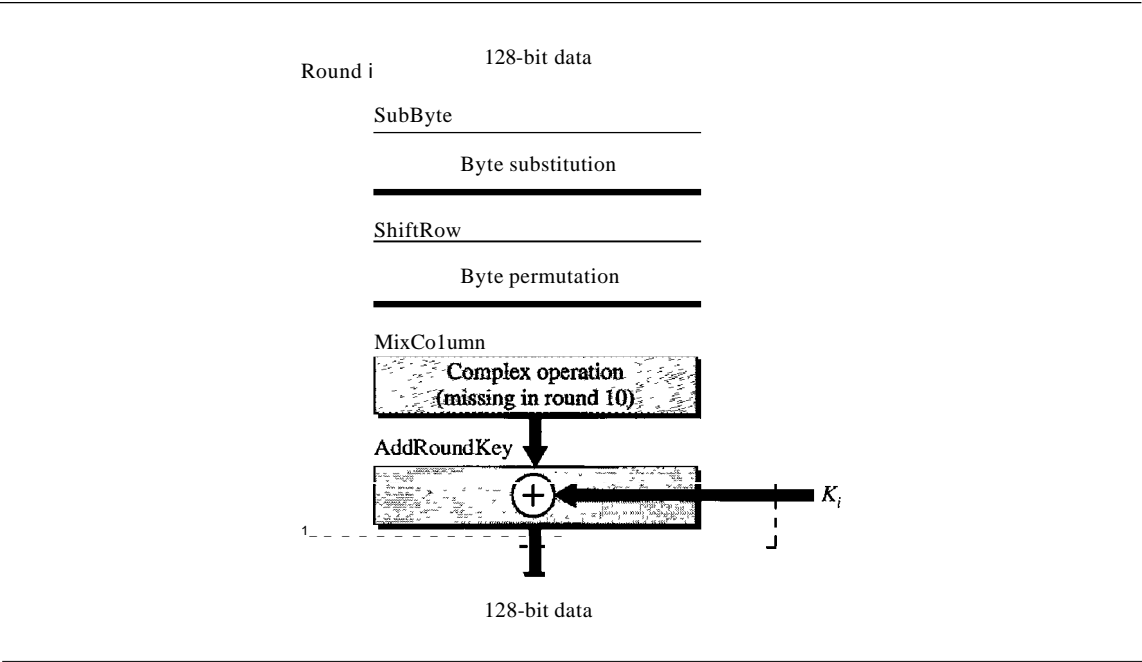
Figure 30.18 Structure of each round
