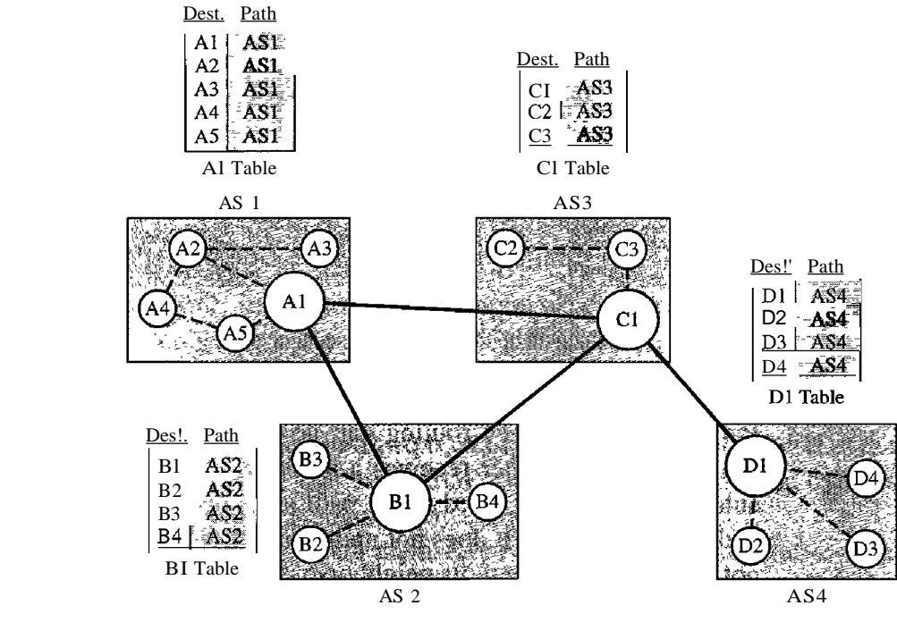
Figure 22.30 Initial routing tables in path vector routing
