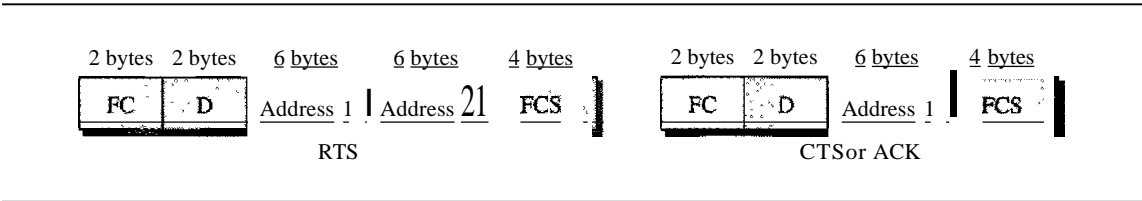
Figure 14.8 Controlframes
