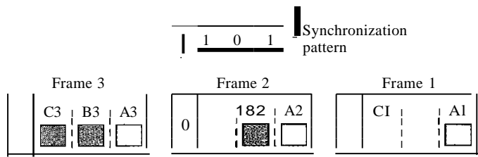
Figure 6.22 Framing bits
