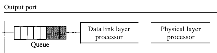
Figure 8.23 Output port
