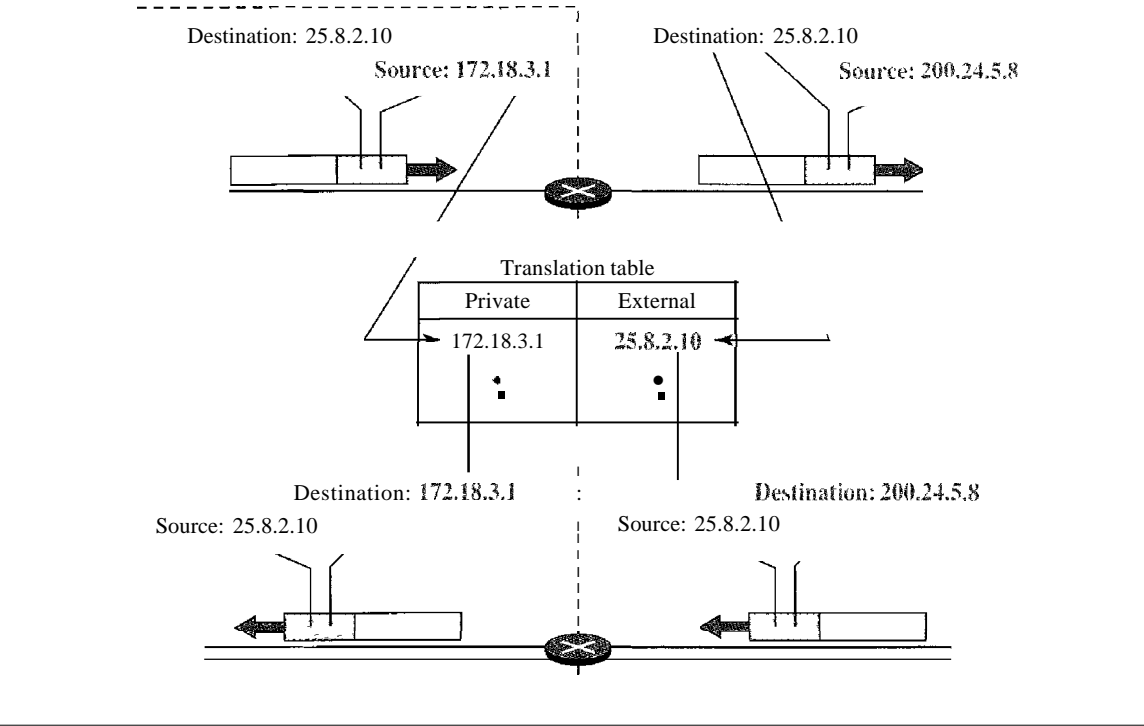
Figure 19.12 NAT address translation
