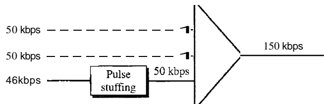
Figure 6.21 Pulse stuffing
