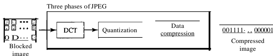
Figure 29.3 JPEG process
