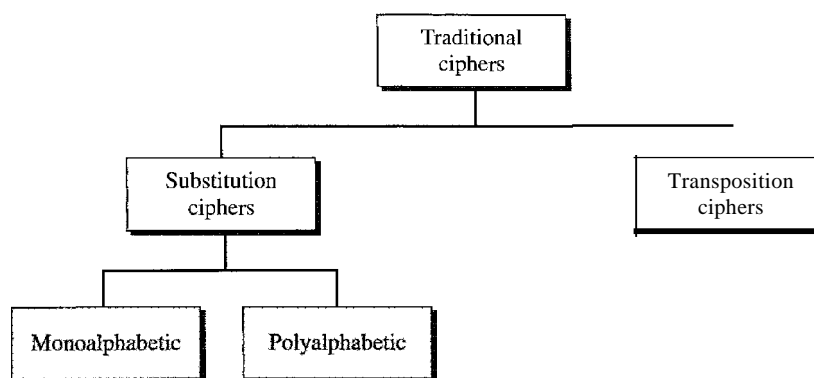
Figure 30.7 Traditional ciphers
