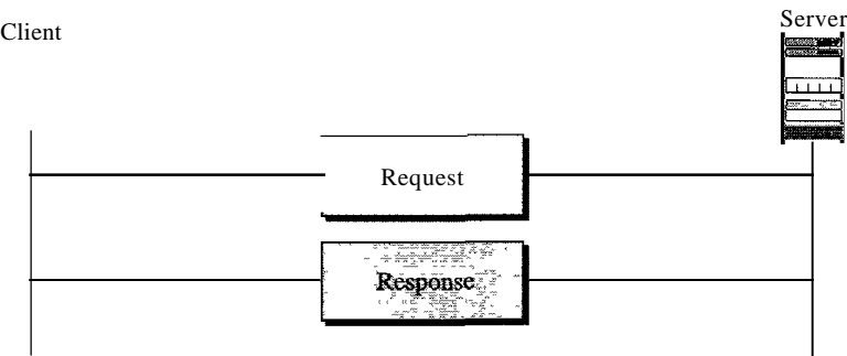
Figure 27.12 HTTP transaction
