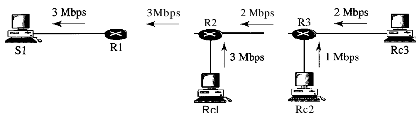
Figure 24.24 Reservation merging
