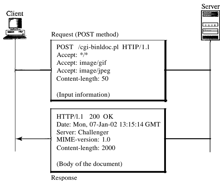
Figure 27.17 Example 27.2
