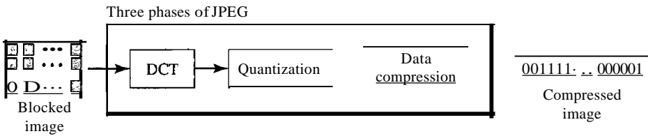
Figure 29.3 JPEG process
