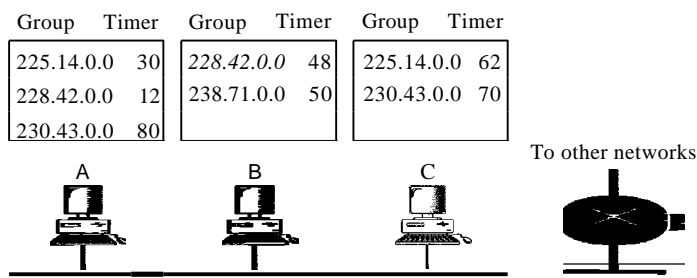
Figure 21.19 Example 21.6
