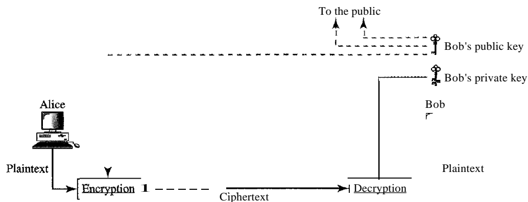
Figure 30.4 Asymmetric-key cryptography
