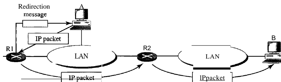
Figure 21.11 Redirection concept
