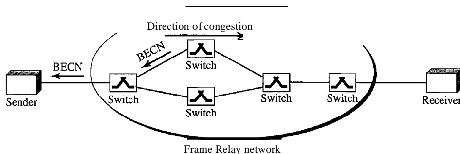
Figure 24.12 BECN
