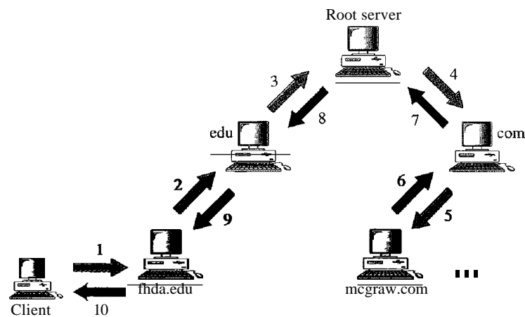
Figure 25.12 Recursive resolution
