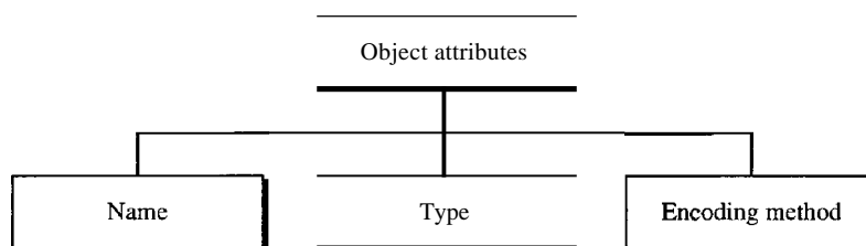
Figure 28.5 Object attributes
