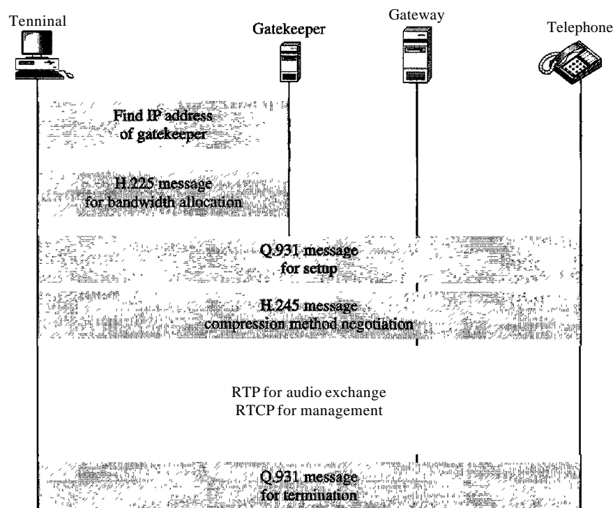
Figure 29.27 H.323 example
