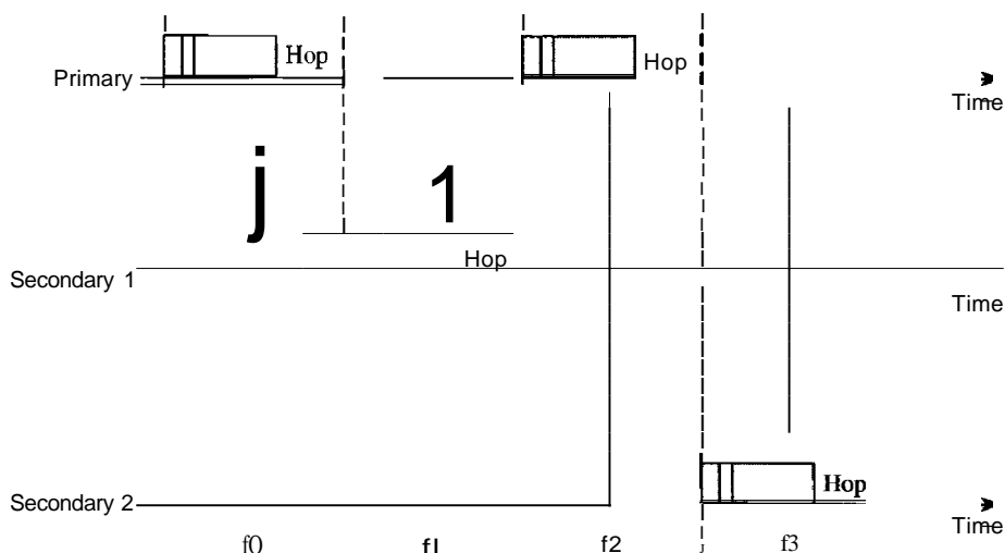
Figure 14.23 Multiple-secondary communication
