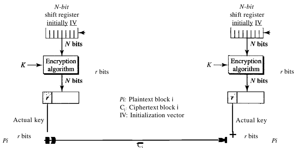
Figure 30.23 OFB mode
