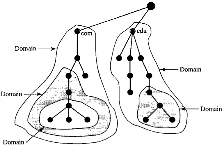
Figure 25.5 Domains
