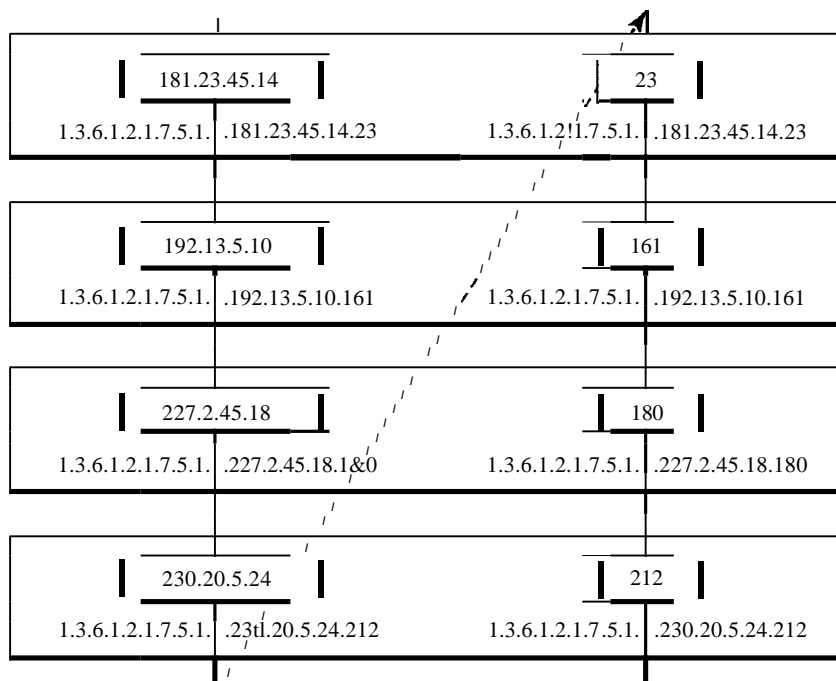
Figure 28.19 Lexicographic ordering
