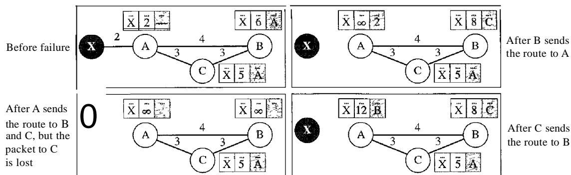
Figure 22.18 Three-node instability
