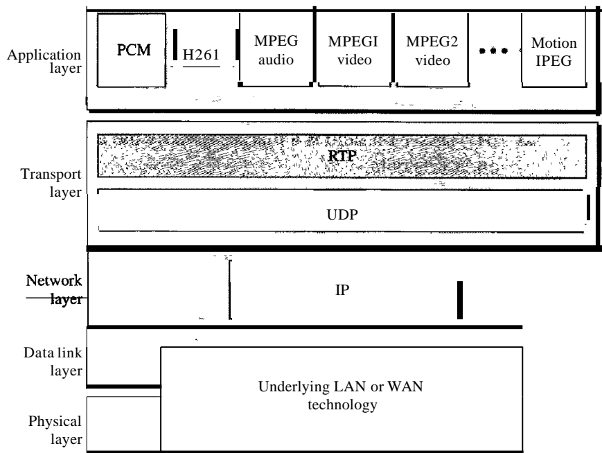
Figure 29.18 RTP
