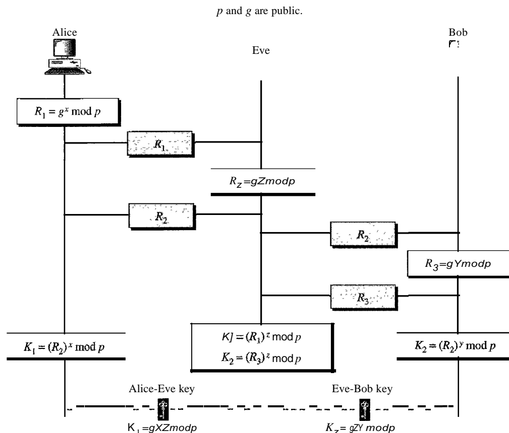
Figure 30.28 Man-in-the-middle attack
