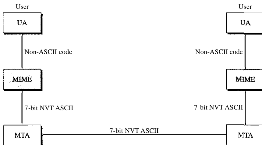
Figure 26.14 MIME
