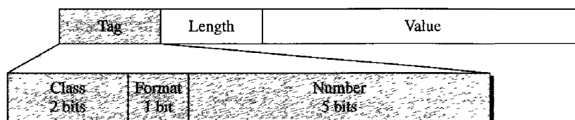
Figure 28.9 Encoding format
