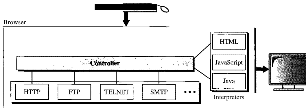
Figure 27.2 Browser
