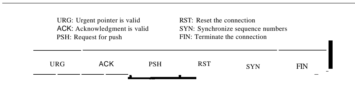
Figure 23.17 Control field
