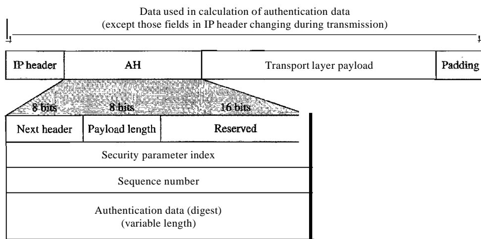
Figure 32.6 Authentication Header (AH) Protocol in transport mode
