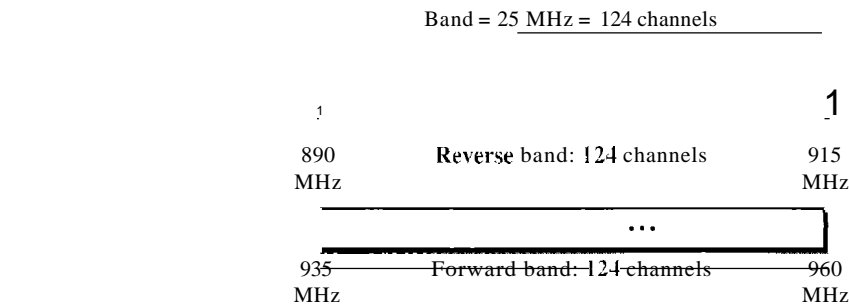
Figure 16.7 GSM bands
