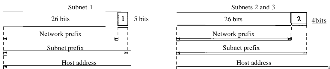
Figure 19.8 Three-level hierarchy in an IPv4 address
