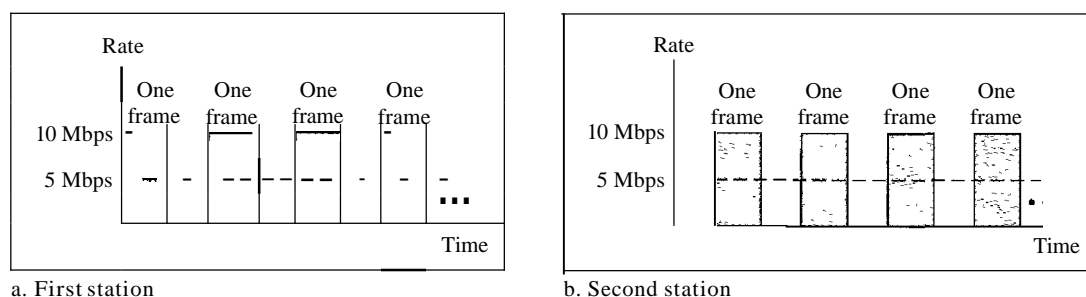
Figure 13.14 Sharing bandwidth
