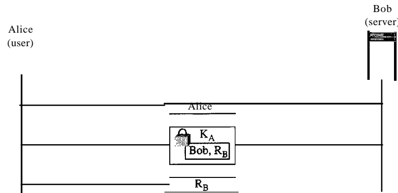
Figure 31.17 Authentication, asymmetric-key
