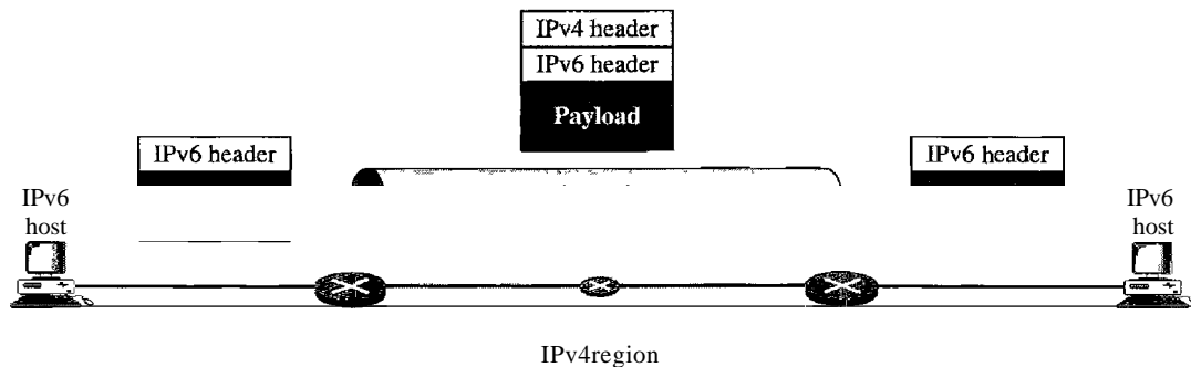
Figure 20.20 Tunneling strategy
