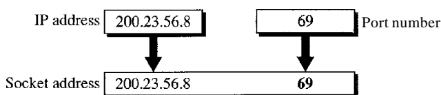
Figure 23.5 Socket address
