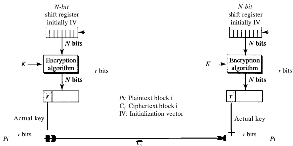
Figure 30.23 OFB mode
