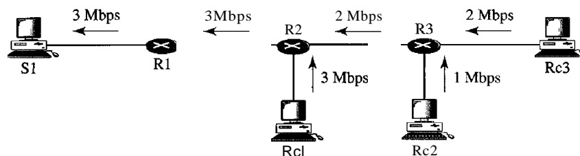
Figure 24.24 Reservation merging
