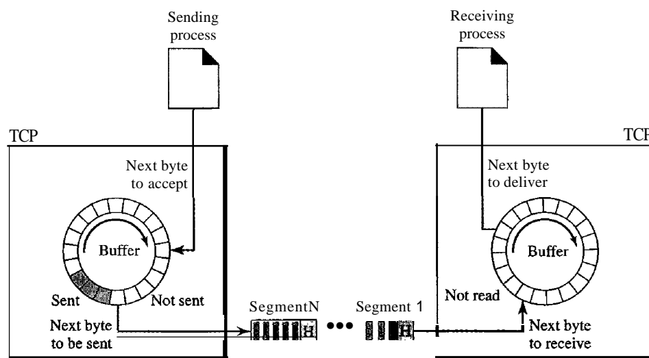
Figure 23.15 TCP segments
