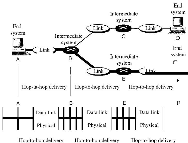
Figure 2.7 Hop-to-hop delivery
