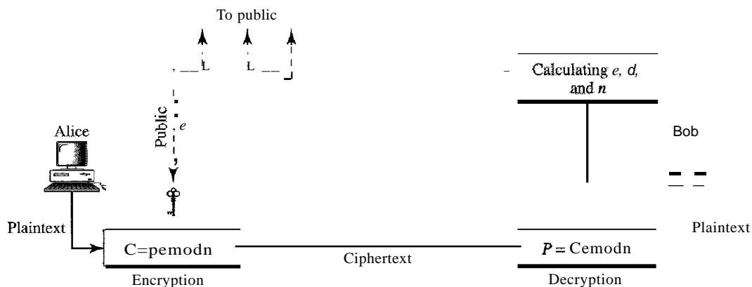
Figure 30.24 RSA
