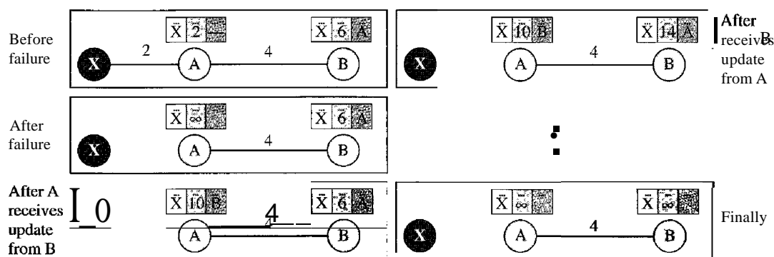
Figure 22.17 Two-node instability
