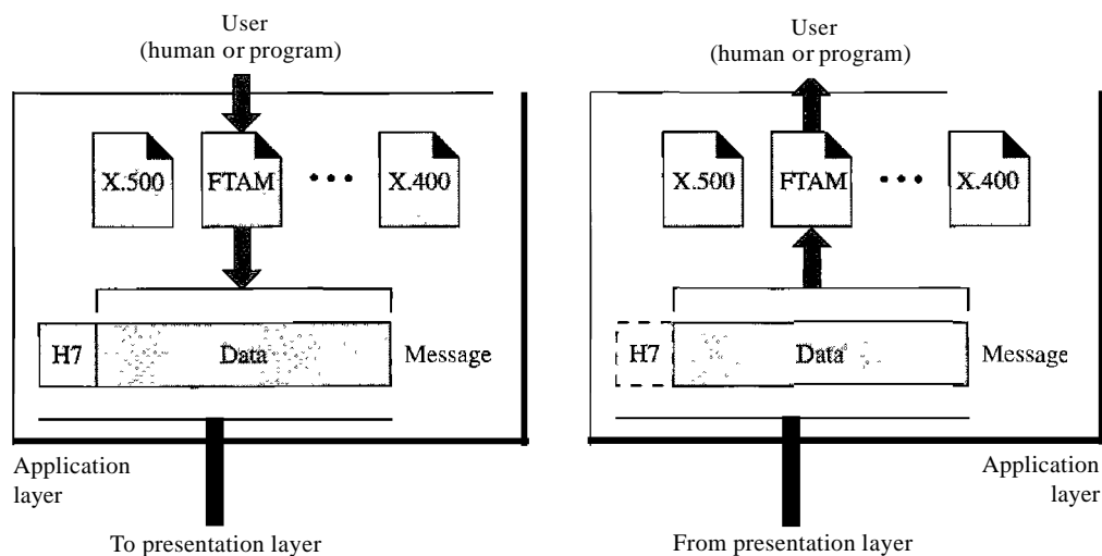
Figure 2.14 Application layer
