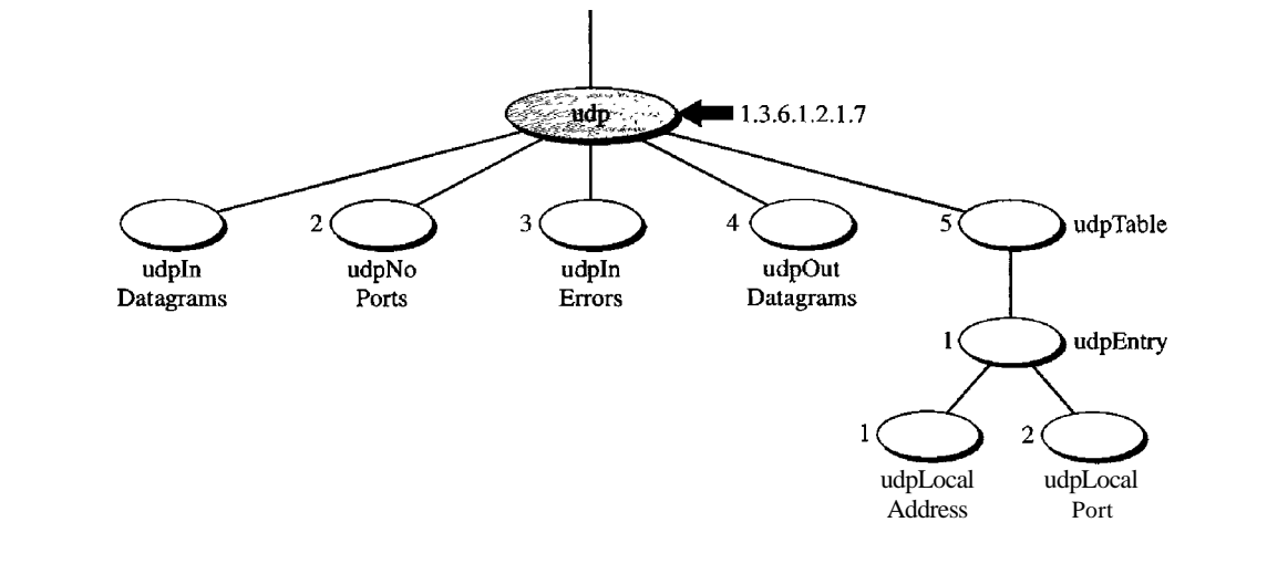
Figure 28.16 udp group
