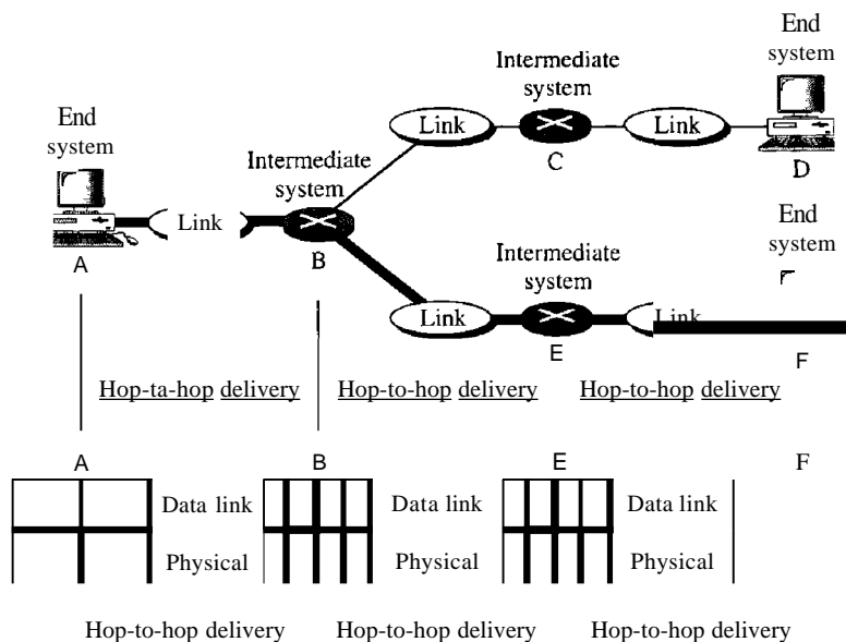
Figure 2.7 Hop-to-hop delivery
