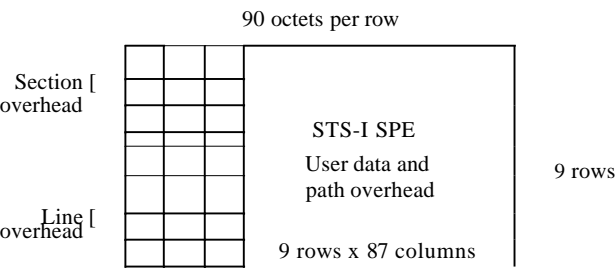
Figure 17.6 STS-1 frame overheads
