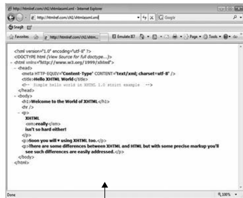
Parse Tree
