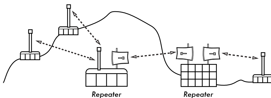
Figure 3.23: No power was available at the top of the hill, but it was circumvented by using multiple repeater sites around the base.
