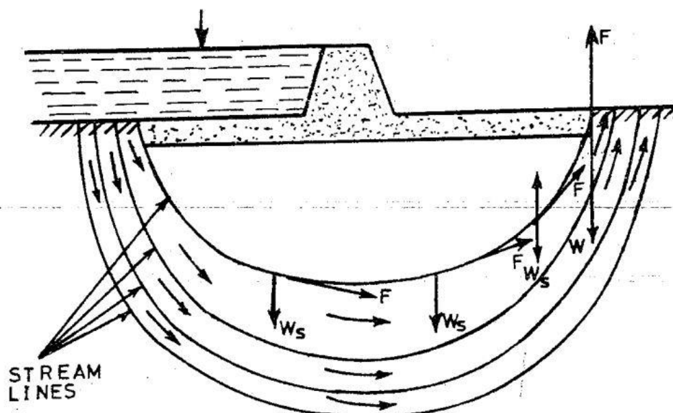
شکل 3.6: Stream lines Under Weir
