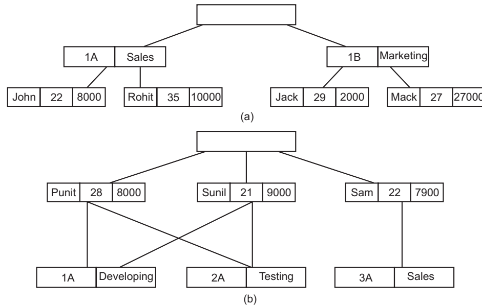
FIGURE 4.6. Sample database.
