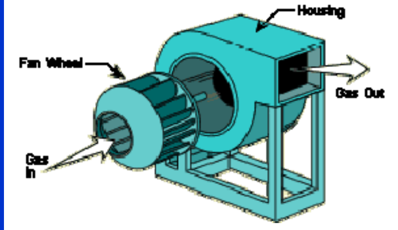
Figure 2. Centrifugal Fan Components
