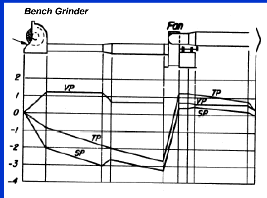
Pressure Graphs for TP, SP, and VP
