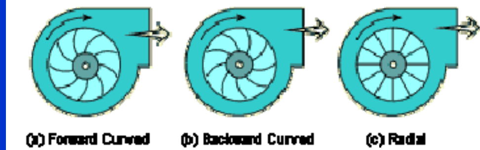
Figure 4. Types of Fan Wheels:
