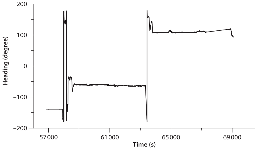
Fig. 10.15. Heading determined by GPS
