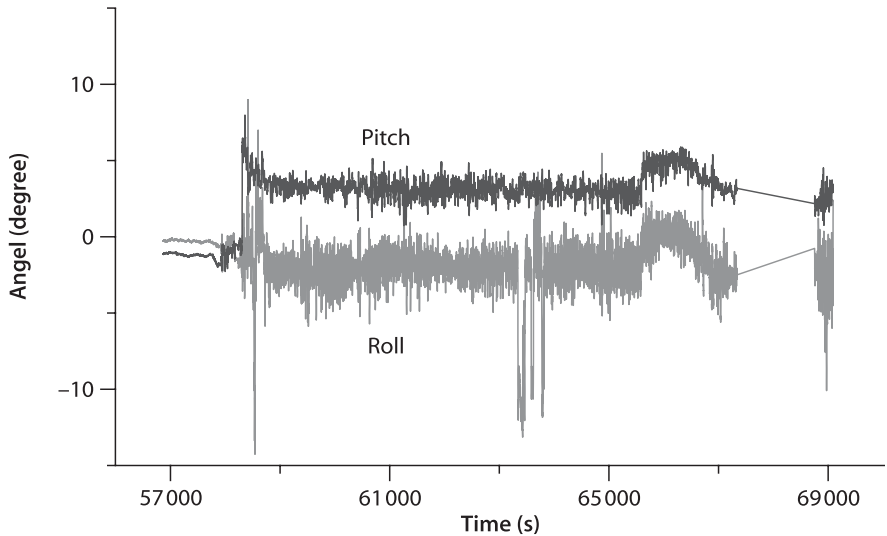
Fig. 10.16. Pitch and roll determined by GPS
