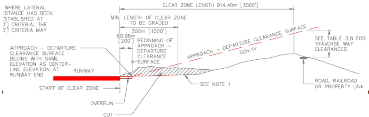
OVERRUN CUT PROFILE
