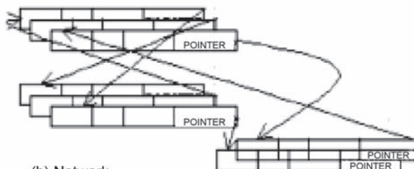
(b) Network
