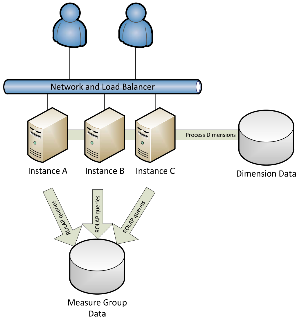
Figure 74 - ROLAP scale-out
