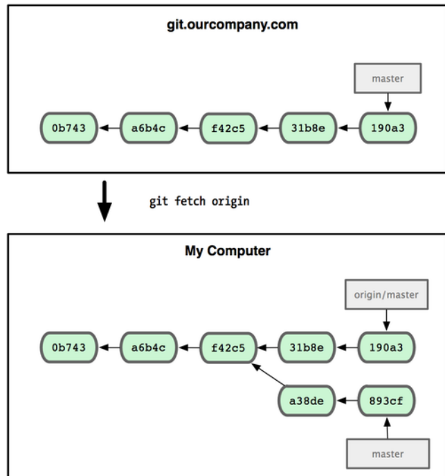
Figure 3.24: The git fetch command updates your remote references.
