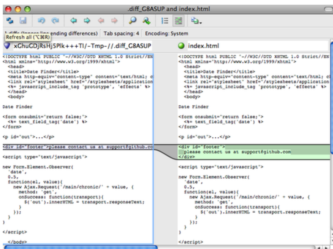
Figure 7.1: P4Merge.
