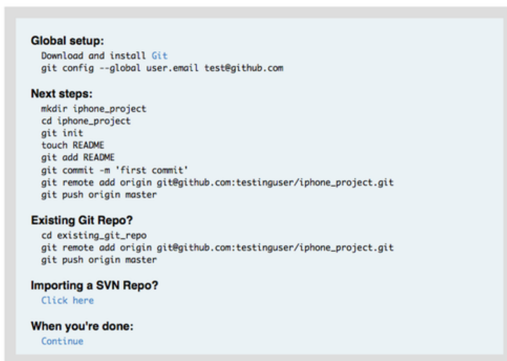
Figure 4.7: Instructions for a new repository.
