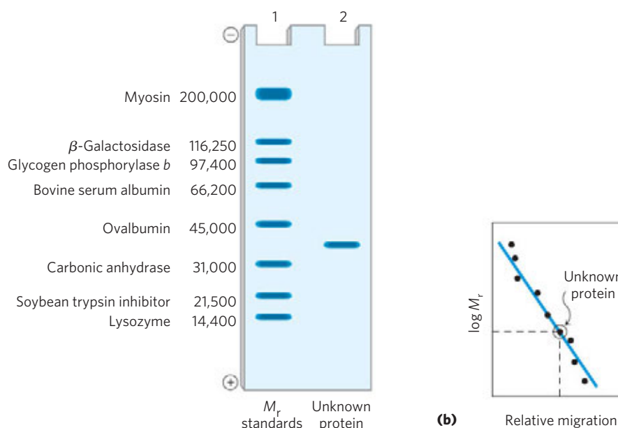
FIGURE 3-19 Estimating the molecular weight of a protein. The electrophoretic mobility of a protein on an SDS polyacrylamide gel is related to its molecular weight, M_r . (a) Standard proteins of known molecular weight are subjected to electrophoresis (lane 1). These marker proteins can be used to estimate the molecular weight of an unknown protein (lane 2). (b) A plot of \log M_r of the marker proteins versus relative migration
