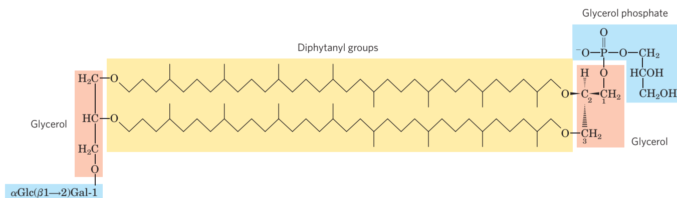
FIGURE 10-12 An unusual membrane lipid found only in some archaea.
