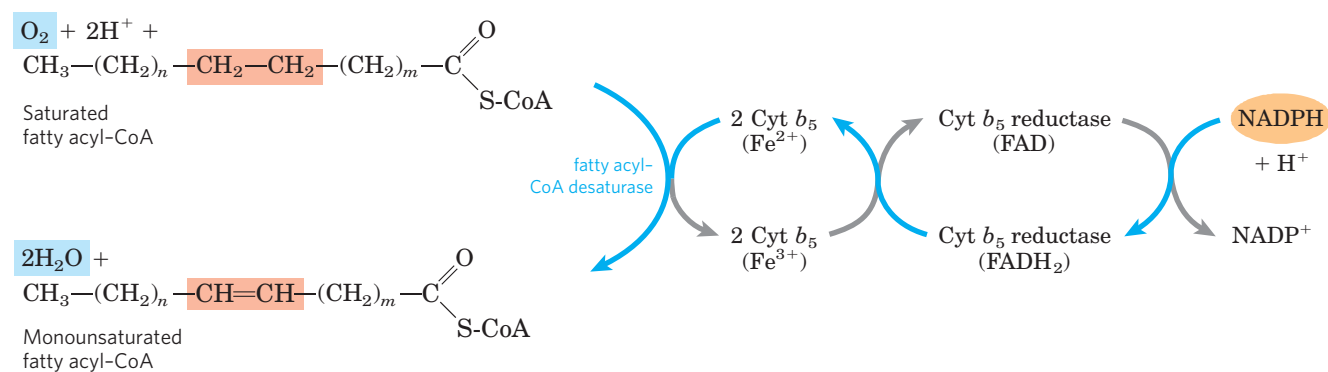
FIGURE 21-13 Electron transfer in the desaturation of fatty acids in vertebrates. Blue arrows show the path of electrons as two substrates—a fatty acyl-CoA and NADPH—undergo oxidation by molecular oxygen.
