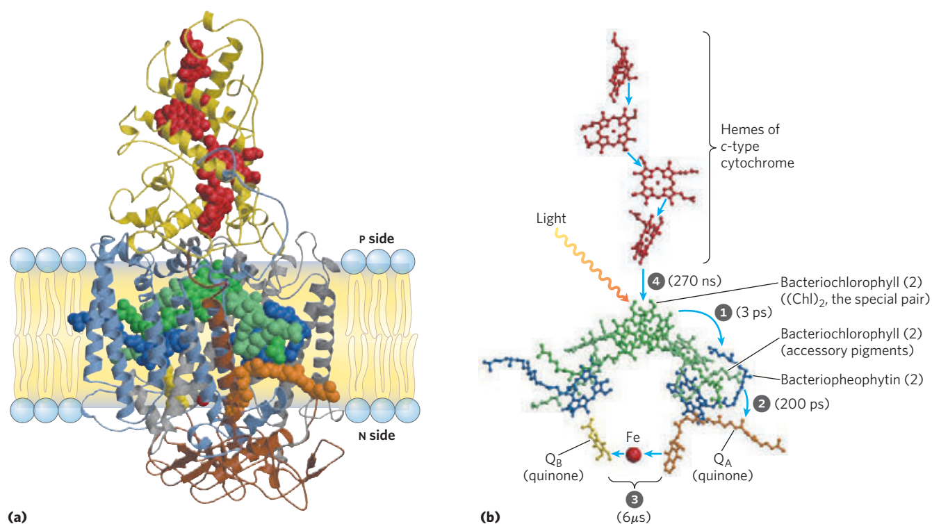
FIGURE 19-57 Photoreaction center of the purple bacterium Rhodospseudomonas viridis . (PDB ID 1PRC) (a) The system has four components: three subunits, H, M, and L (brown, blue, and gray, respectively), with a total of 11 transmembrane helical segments, and a fourth protein, cytochrome c (yellow), associated with the complex at the membrane surface. Subunits L and M are paired transmembrane proteins that together form a cylindrical structure with roughly bilateral symmetry about its long axis. Shown as space-filling models (and in (b) as ball-and-stick structures) are the prosthetic groups that participate in the photochemical events. Bound to the L and M chains are two pairs of bacteriochlorophyll molecules (green); one of the pairs—the “special pair,” (\text{Chl})_2 —is the site of the first photochemical changes after light absorption. Also incorporated in the system are a pair of pheophytin a (Pheo a ) molecules (blue); two
