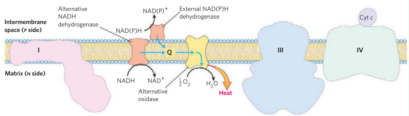
FIGURE 2 Electron carriers of the inner membrane of plant mitochondria. Electrons can flow through Complexes I, III, and IV, as in
