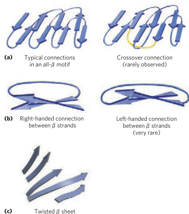
FIGURE 4-20 Stable folding patterns in proteins. (a) Connections between \beta strands in layered \beta sheets. The strands here are viewed from one end, with no twisting. The strands here are viewed from the ends nearest the viewer; thick lines are connections at the ends nearest the viewer; thin lines are connections at the far ends of the \beta strands. The connections at a given end (e.g., near the viewer) rarely cross one another. An example of such a rare crossover is illustrated by the yellow strand in the structure on the right. (b) Because of the right-handed twist in \beta strands, connections between strands are generally right-handed. Left-handed connections must traverse sharper angles and are harder to form. (c) This twisted \beta sheet is from a domain of photolyase (a protein that repairs certain types of DNA damage) from E. coli (derived from PDB ID 1DNP). Connecting loops have been removed so as to focus on the folding of the \beta sheet.
