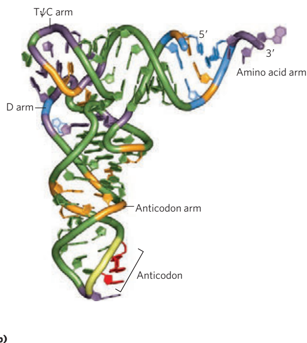
than sequence are important for recognition by some of the synthetases. (b) (PDB ID 1EHZ) The same structural features are shown in three dimensions, with the orange and blue residues again representing positions recognized by one or more aminoacyl-tRNA synthetases, respectively.
