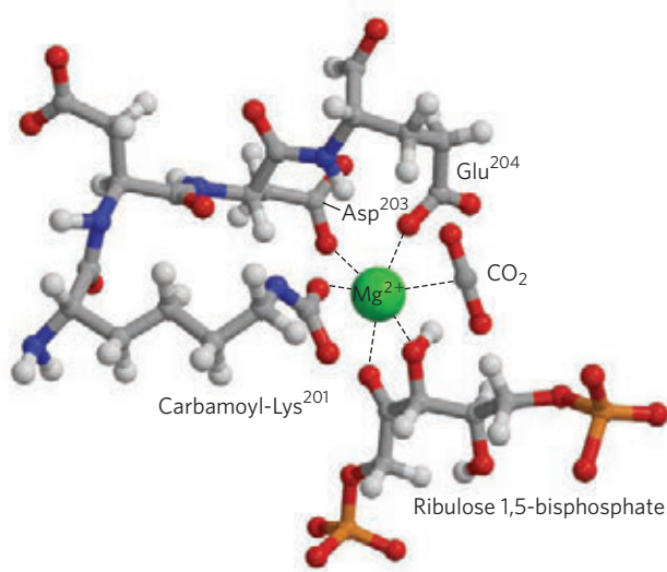
FIGURE 20-6 Central role of Mg^{2+} in the catalytic mechanism of rubisco . (Derived from PDB ID 1RXO) Mg^{2+} is coordinated in a roughly octahedral complex with six oxygen atoms: one oxygen in the carbamate on Lys 201 ; two in the carboxyl groups of Glu 204 and Asp 203 ; two at C-2 and C-3 of the substrate, ribulose 1,5-bisphosphate; and one in the other substrate, CO 2 . A water molecule occupies the CO 2 -binding site in this crystal structure. In this figure a CO 2 molecule is modeled in its place. (Residue numbers refer to the spinach enzyme.)
