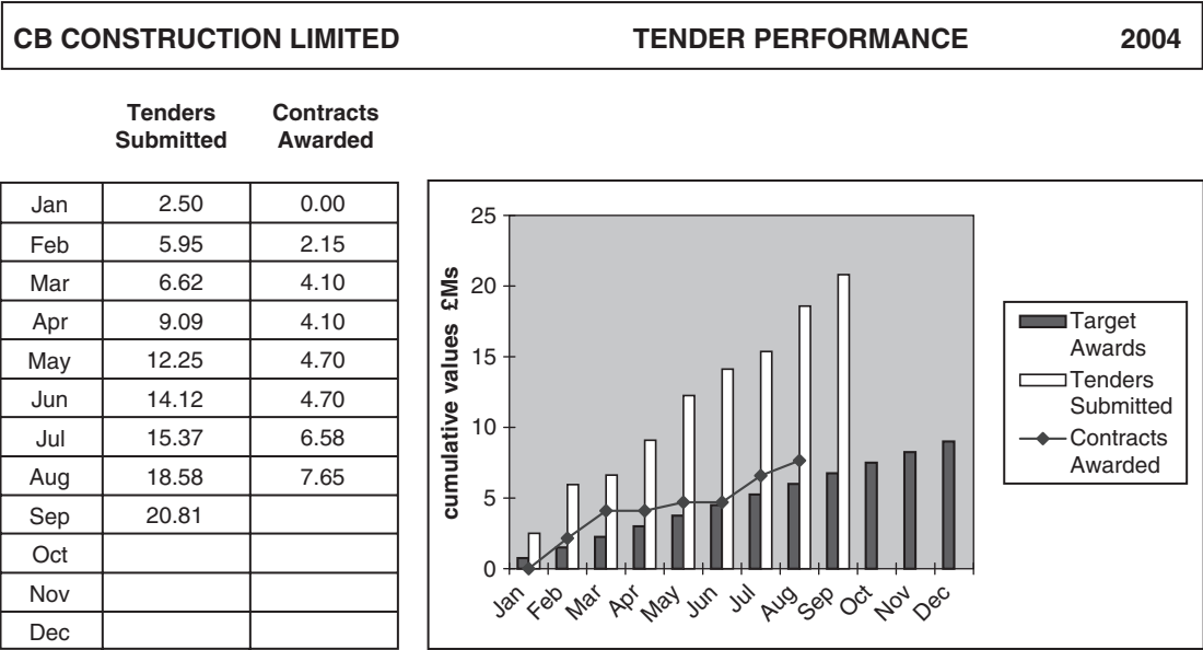
Fig. 18.2 Cumulative value of tenders and awards
