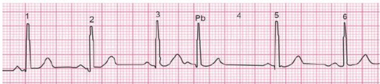
Fig. 8.1: Premature beats
