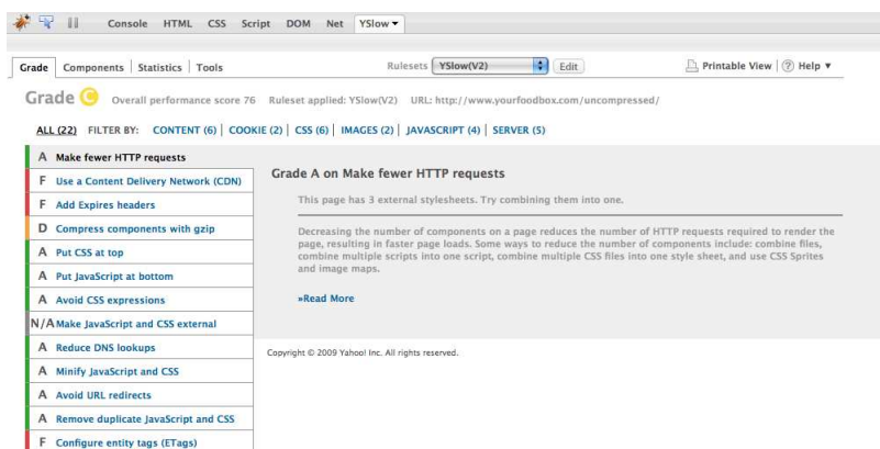
Figure 20.1: YSlow found several problems we might want to address.
