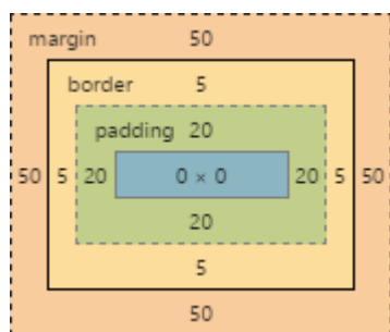
Screenshot of Google Chrome's Element Styles panel
