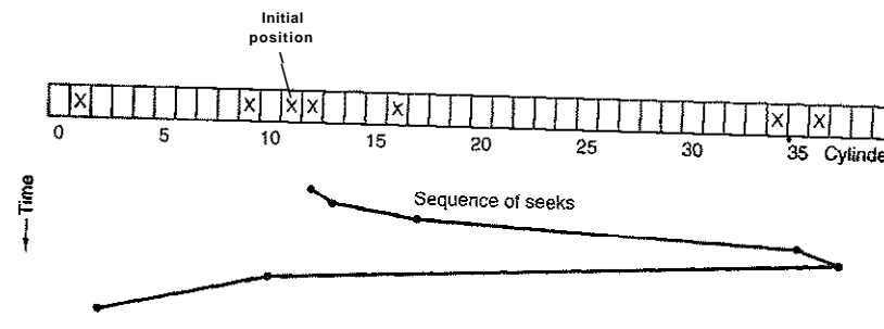
Figure 5-29. The elevator algorithm for scheduling disk requests.
