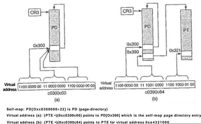
Figure 11-34. The Windows self-map entry used to map the physical pages of the page tables and page directory into kernel virtual addresses, for the x86.
