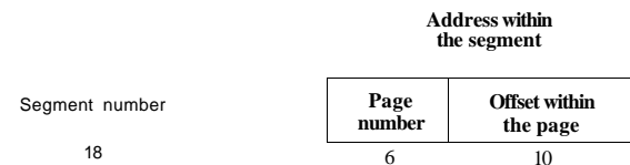
Figure 3-36.. A 34-bit MULTICS virtual address.
