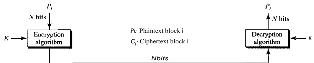
Figure 30.20 ECB mode
