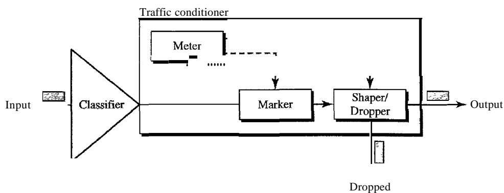
Figure 24.27 Traffic conditioner
