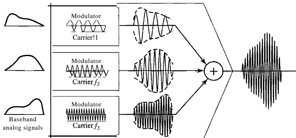
Figure 6.4 FDM process
