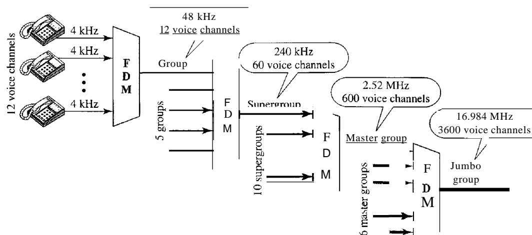
Figure 6.9 Analog hierarchy
