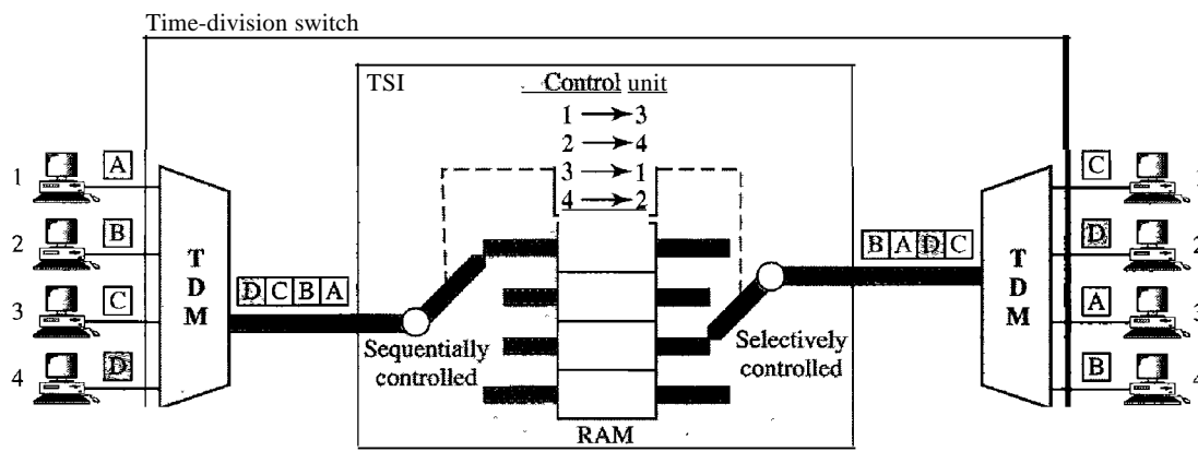
Figure 8.19 Time-slot interchange
