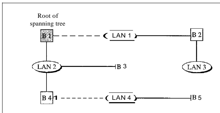
b. Spanning tree
