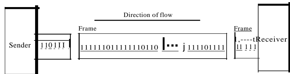
Figure 4.35 Synchronous transmission
