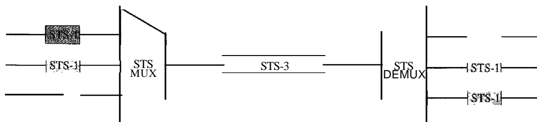
Figure 17.12 STS multiplexing/demultiplexing
