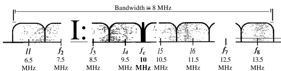
Figure 5.8 Bandwidth of MFSK used in Example 5.6
