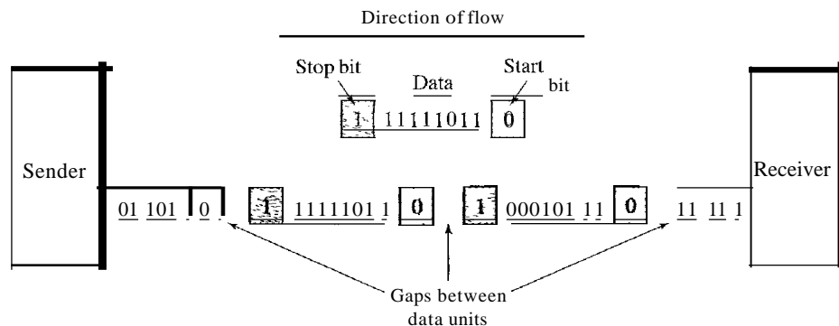
Figure 4.34 Asynchronous transmission
