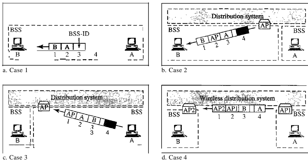
Figure 14.9 Addressing mechanisms
