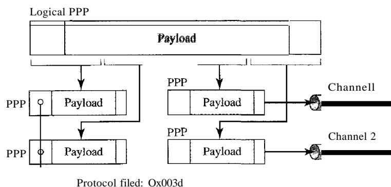
Figure 11.40 Multilink PPP
