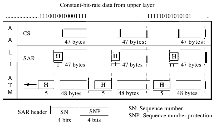
Figure 18.20 AAL1
