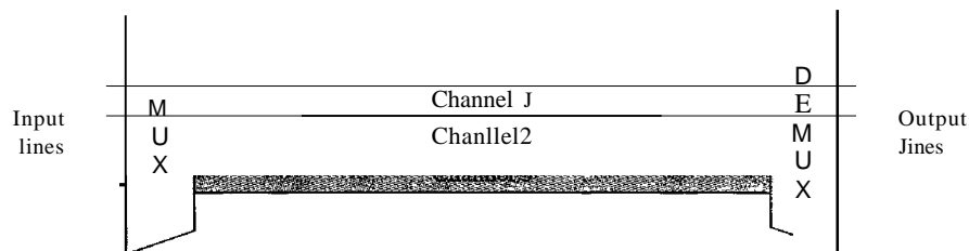
Figure 6.3 Frequency-division multiplexing
