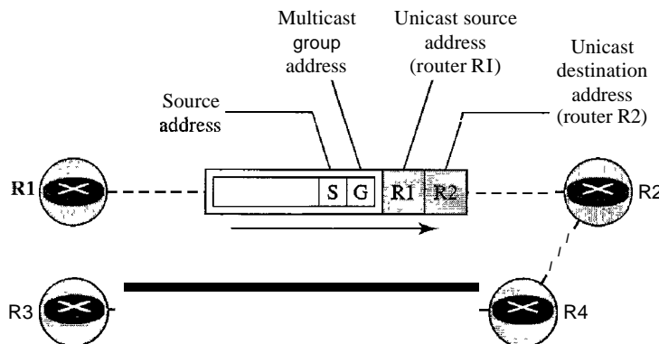
Figure 22.47 MBONE
