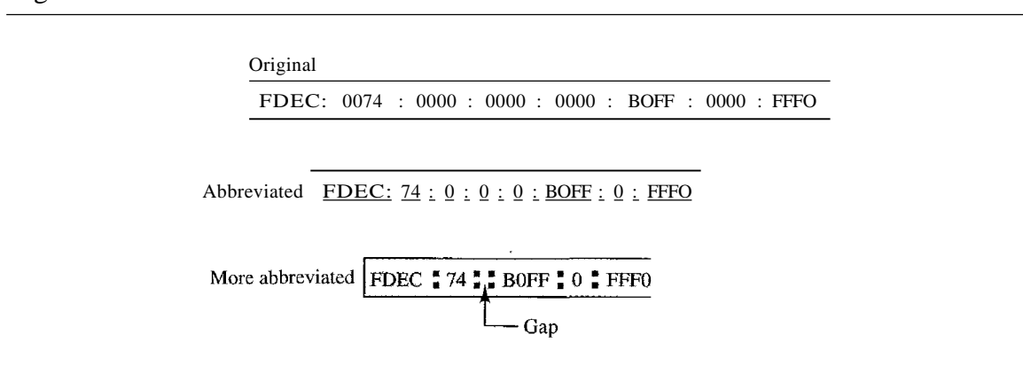
Figure 19.15 Abbreviated IPv6 addresses
