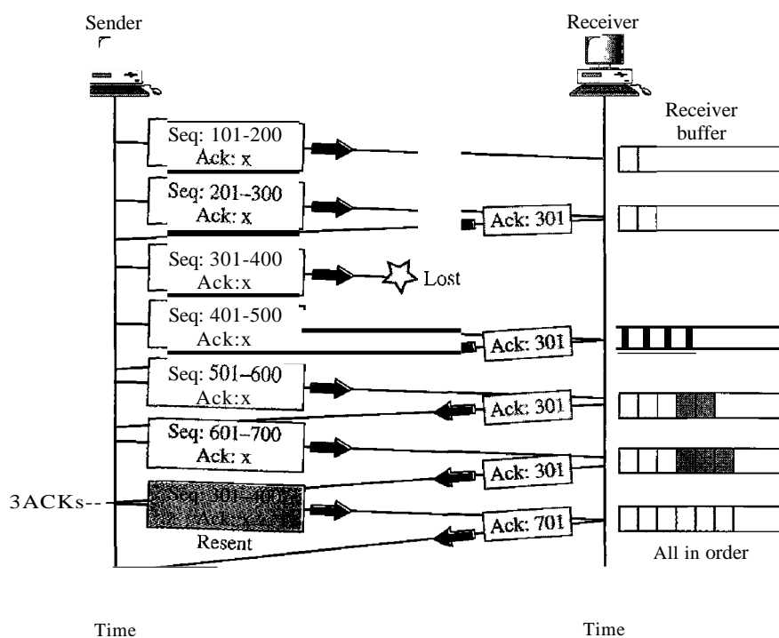
Figure 23.26 Fast retransmission
