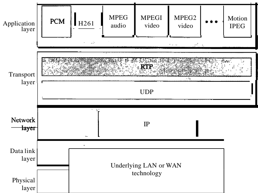
Figure 29.18 RTP
