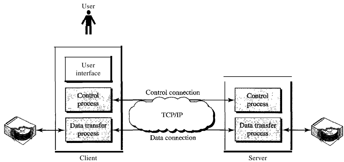
Figure 26.21 FTP
