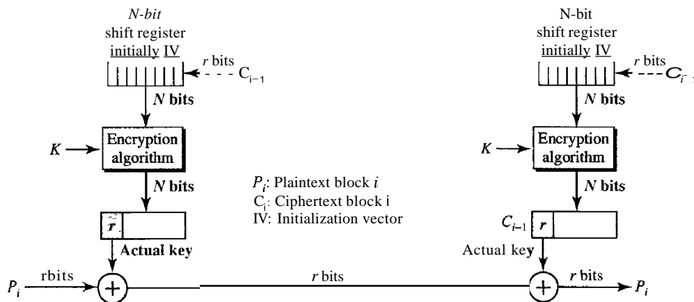
Figure 30.22 CFB mode
