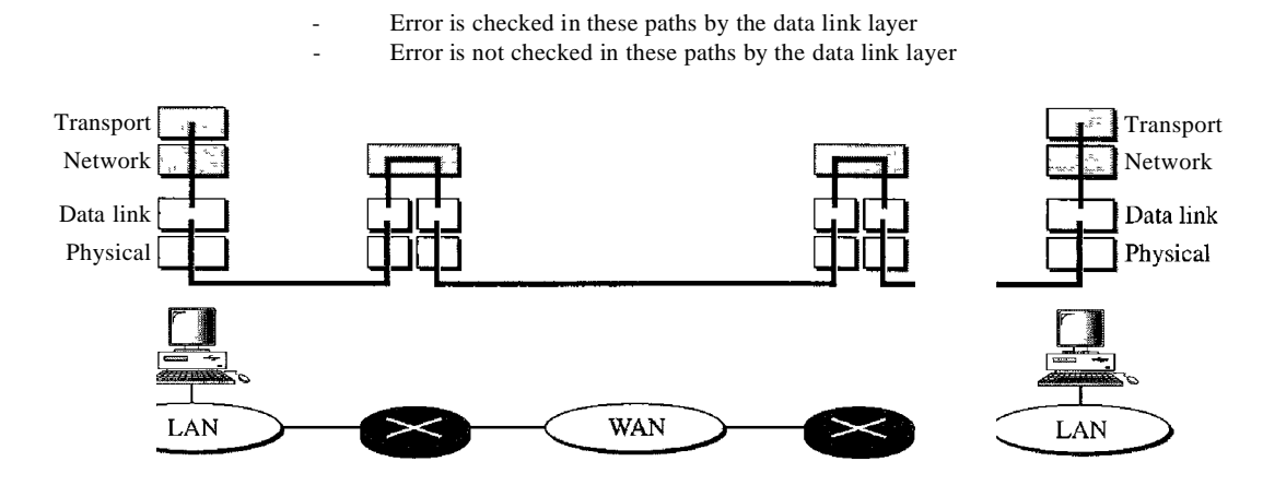
Figure 23.7 Error control
