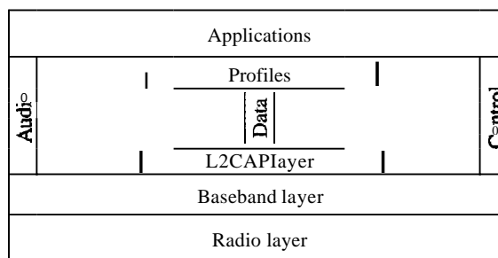
Figure 14.21 Bluetooth layers
