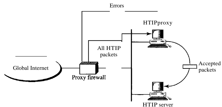
Figure 32.24 Proxy firewall
