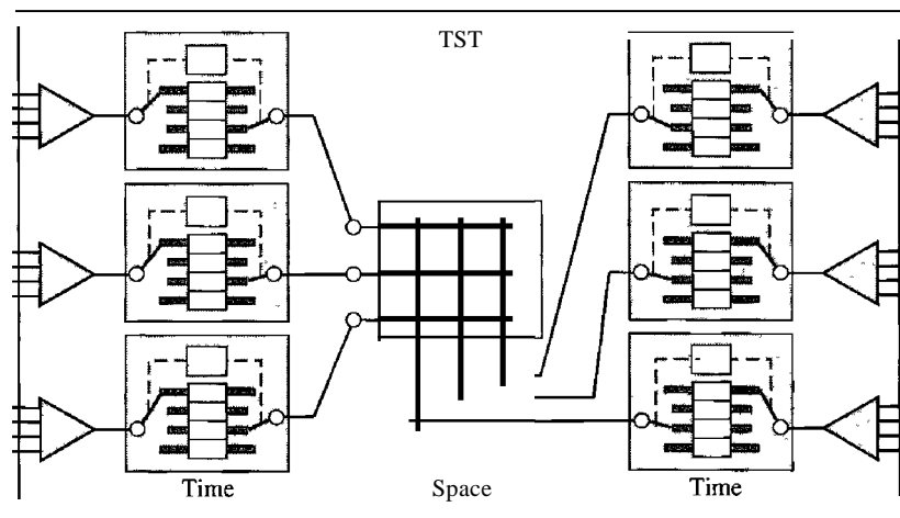
Figure 8.20 Time-space-time switch
