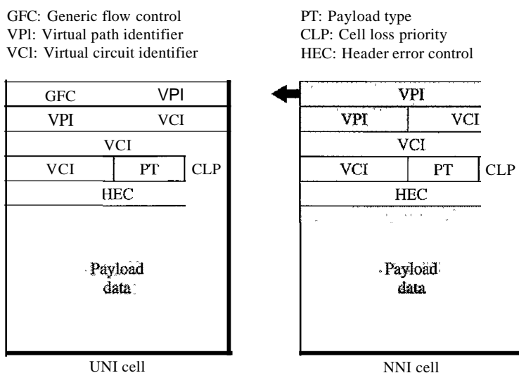
Figure 18.19 ATM headers
