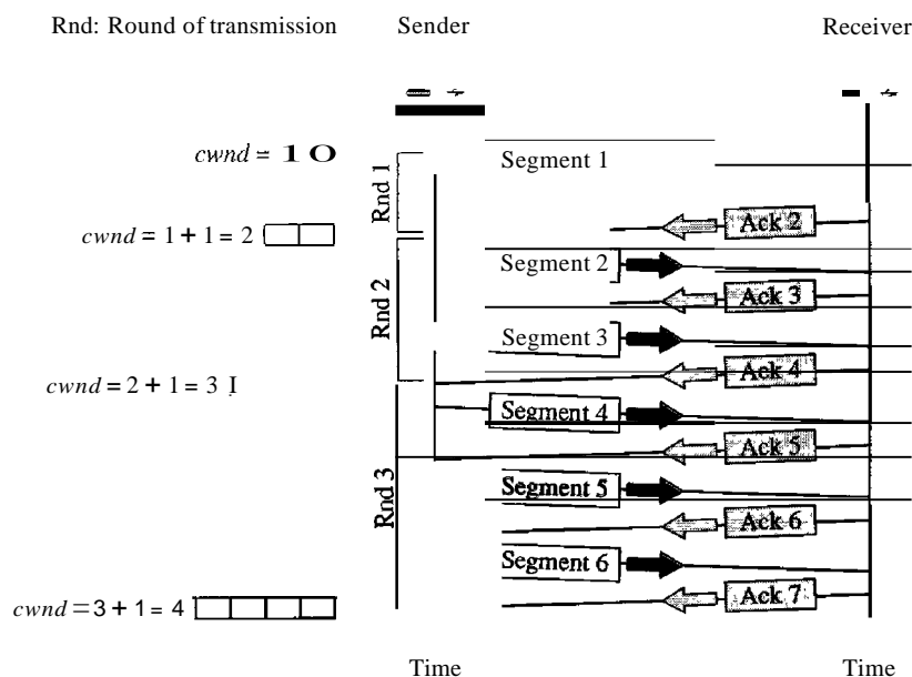
Figure 24.9 Congestion avoidance, additive increase
