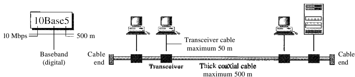
Figure 13.10 10Base5 implementation
