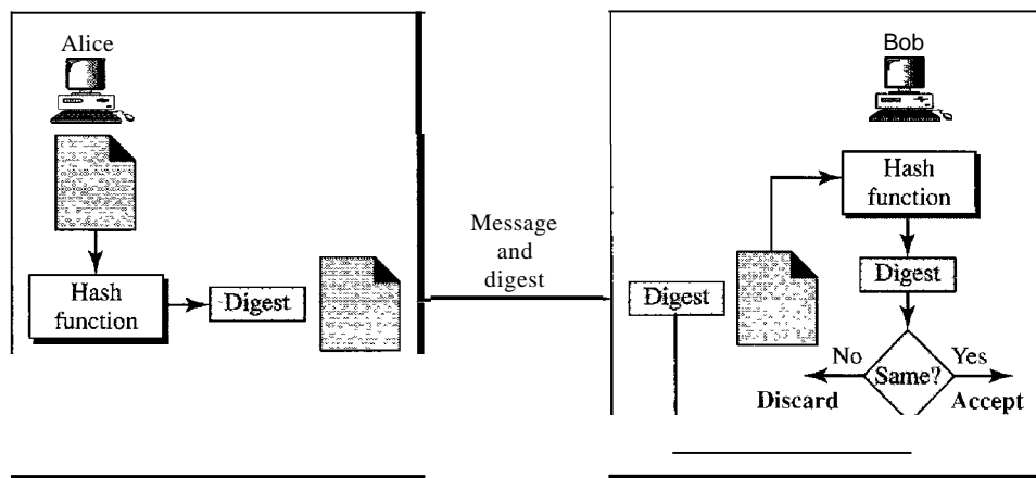
Figure 31.5 Checking integrity
