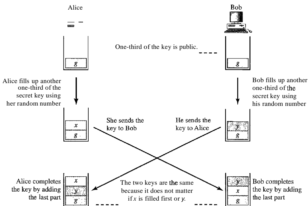
Figure 30.27 Diffie-Hellman idea
