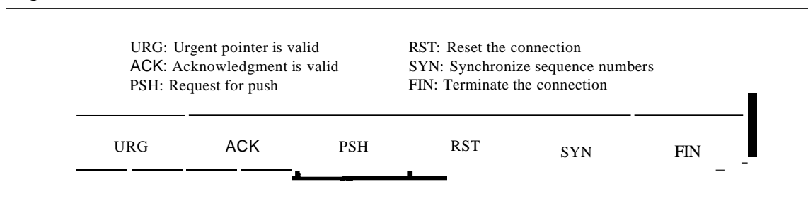
Figure 23.17 Control field
