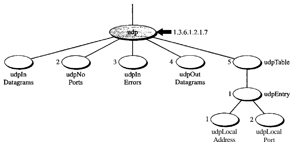
Figure 28.16 udp group
