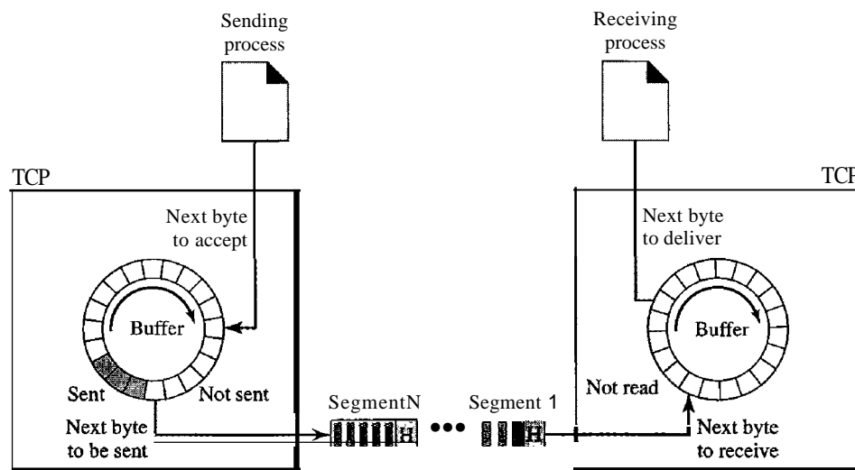
Figure 23.15 TCP segments
