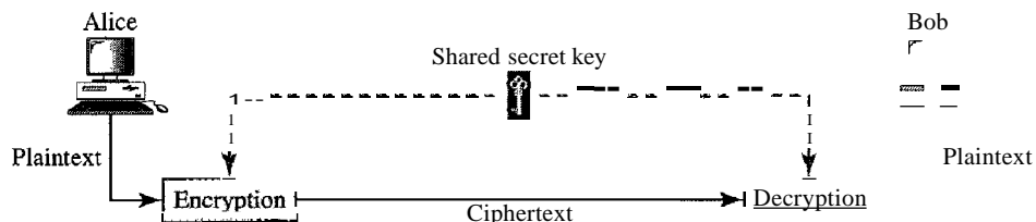
Figure 30.3 Symmetric-key cryptography
