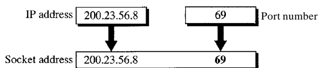
Figure 23.5 Socket address
