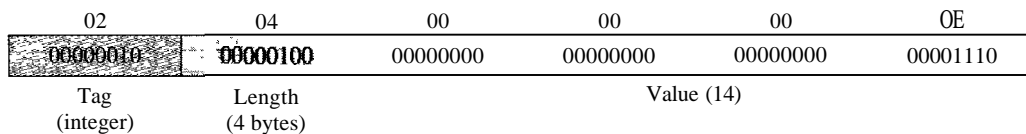
Figure 28.11 Example 28.1, INTEGER 14
