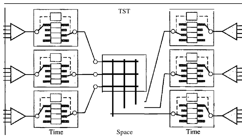
Figure 8.20 Time-space-time switch
