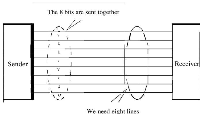
Figure 4.32 Parallel transmission
