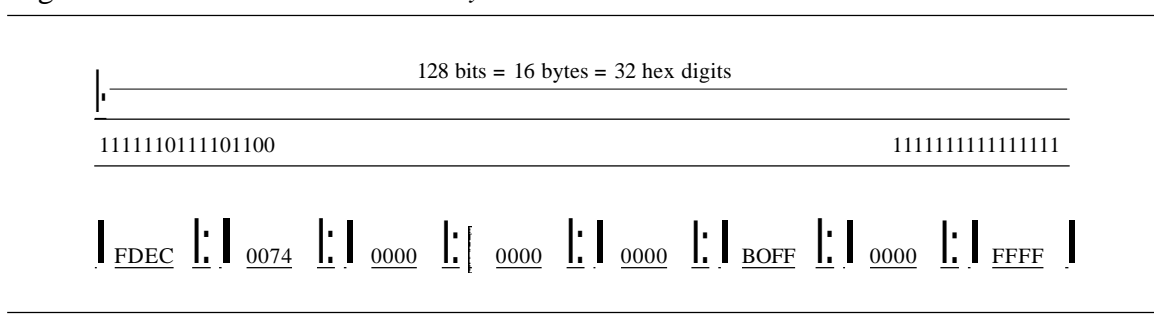
Figure 19.14 IPv6 address in binary and hexadecimal colon notation
