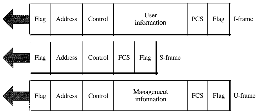
Figure 11.27 HDLC frames
