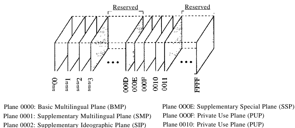
Figure A.2 Unicode planes
