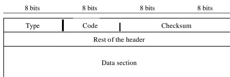
Figure 21.8 General format of ICMP messages
