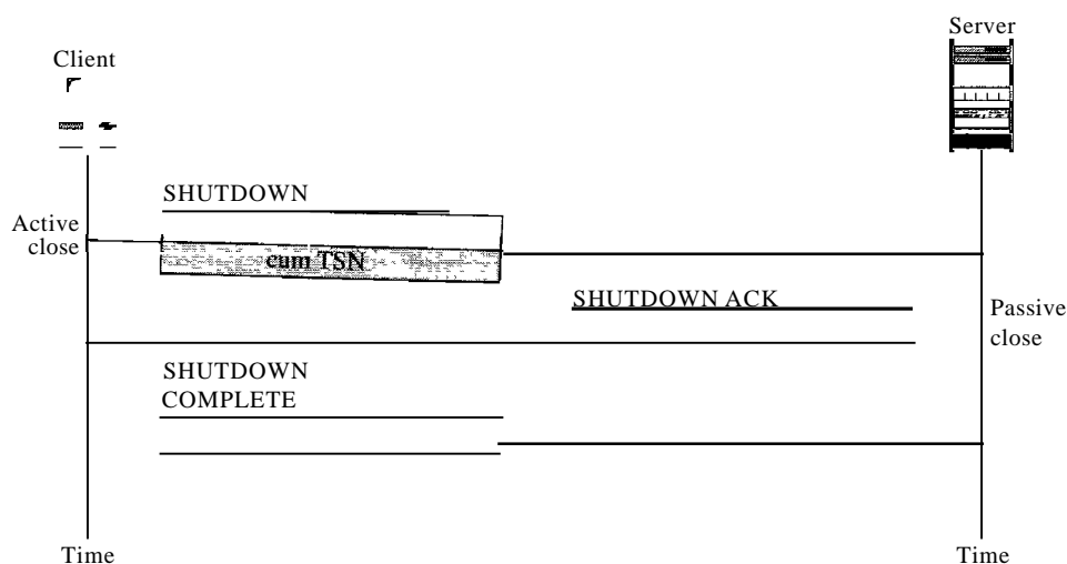
Figure 23.35 Association termination
